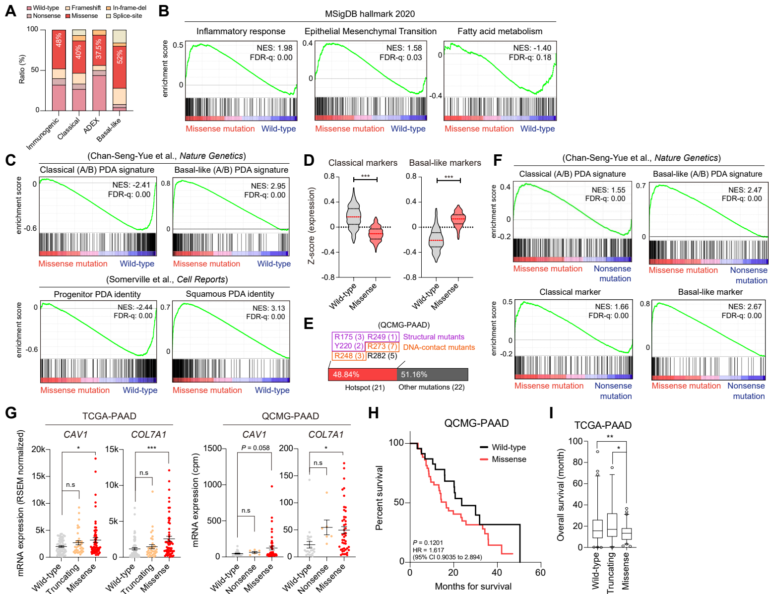
SUPPLEMENTARY FIGURE 3
