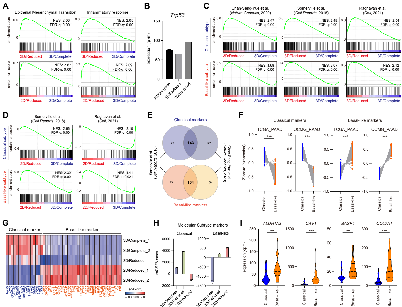
SUPPLEMENTARY FIGURE 2
