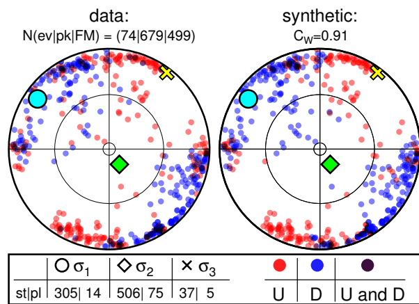
(a) first motions
