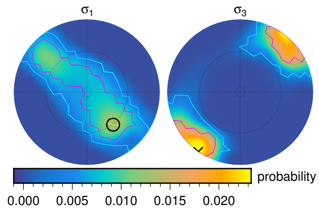
(c) stress axis orientation
