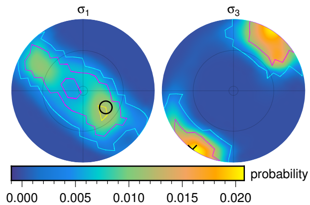
(c) stress axis orientation
