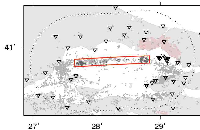
(b) Central Marmara Section (CMS)
