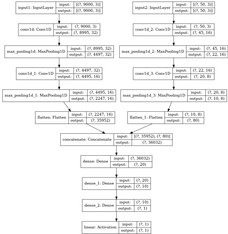
Figure 4: Architecture of Model 3.
