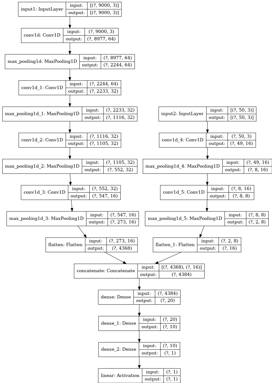
Figure 6: Architecture of Model 5.
