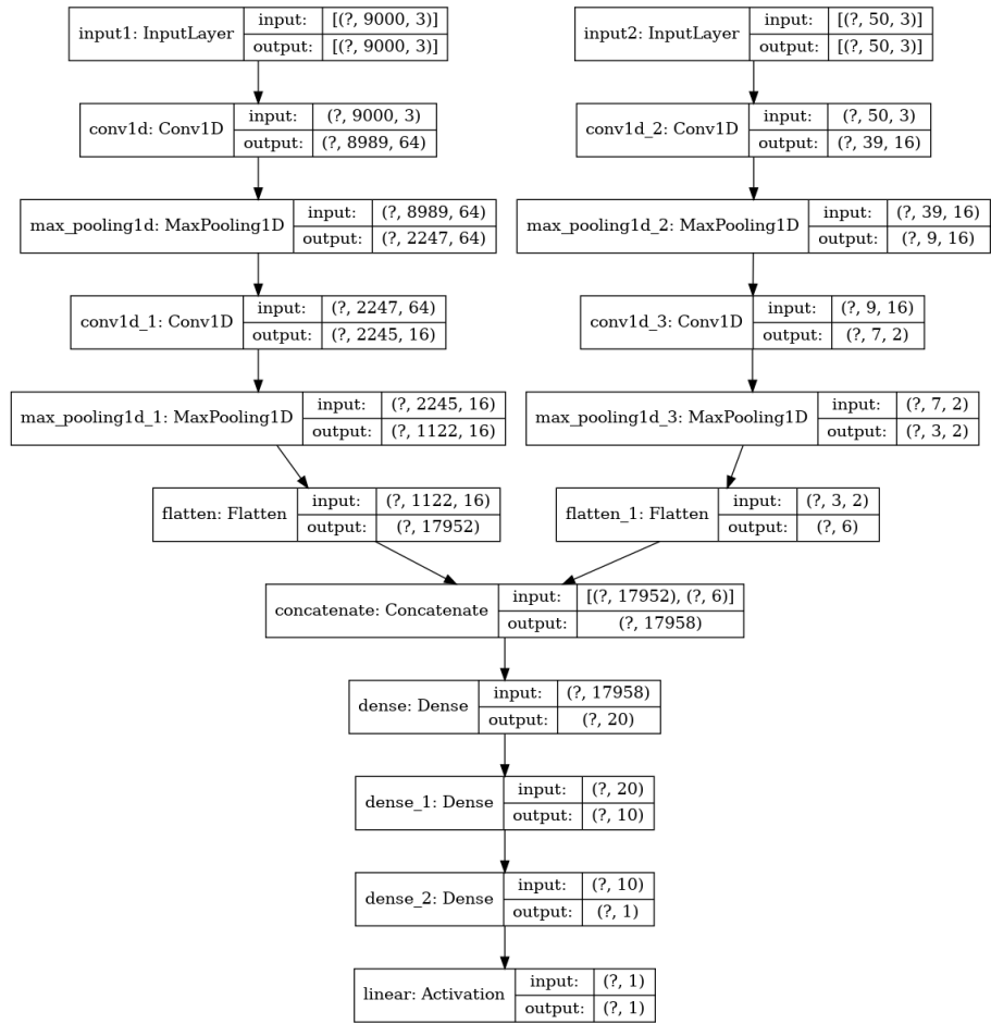
Figure 3: Architecture of Model 2.
