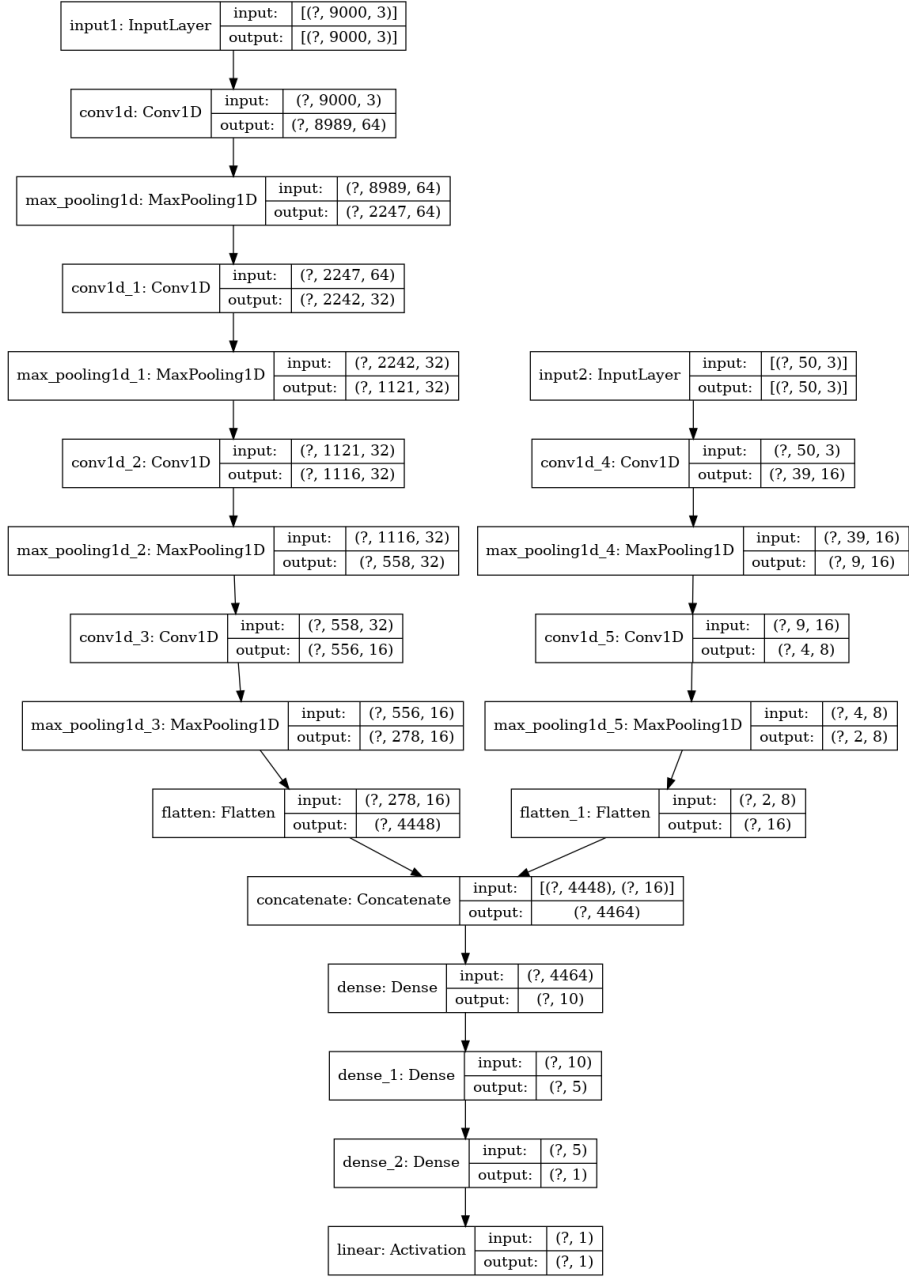
Figure 10: Architecture of Model 9.
