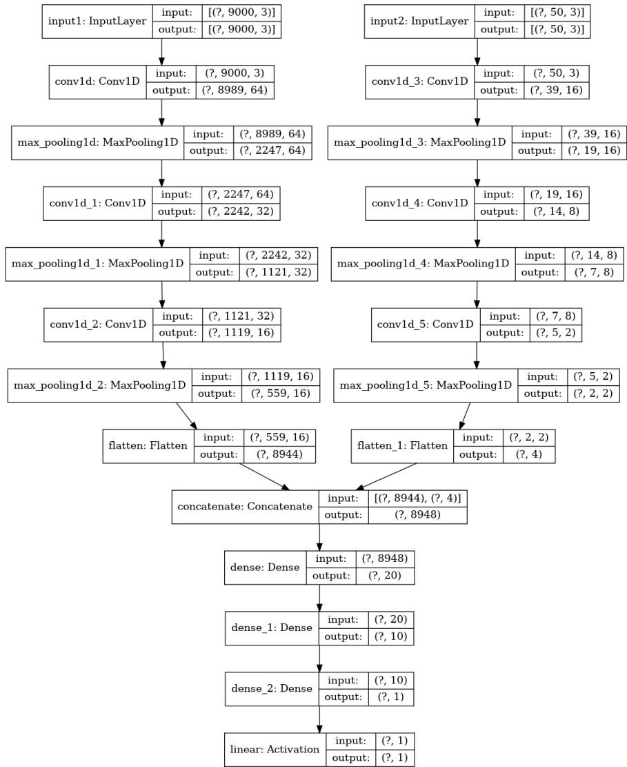
Figure 5: Architecture of Model 4.
