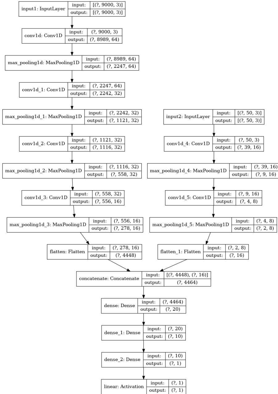
Figure 1: Architecture of Model 0.
