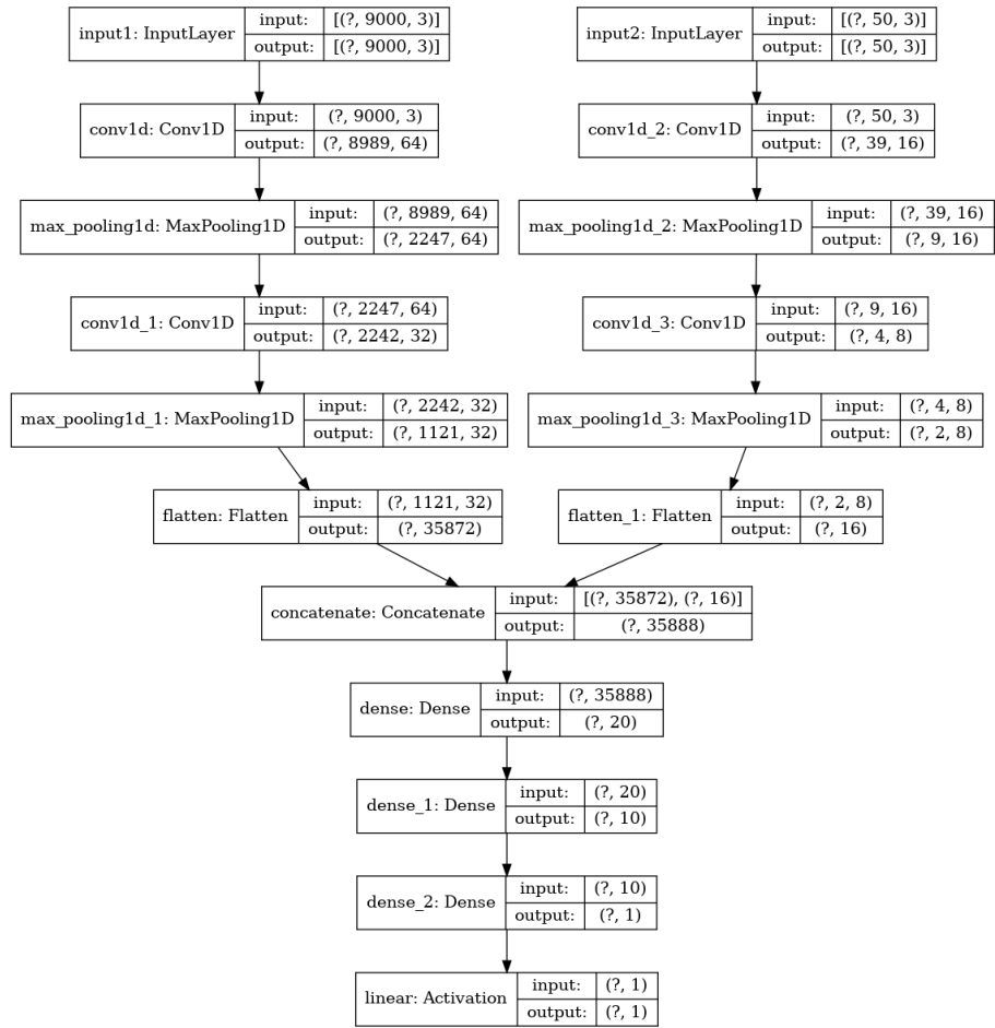
Figure 2: Architecture of Model 1.
