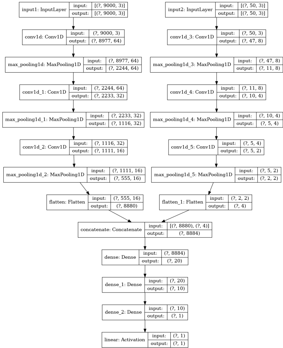
Figure 7: Architecture of Model 6.
