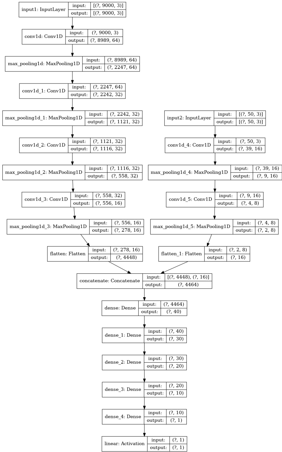
Figure 8: Architecture of Model 7.
