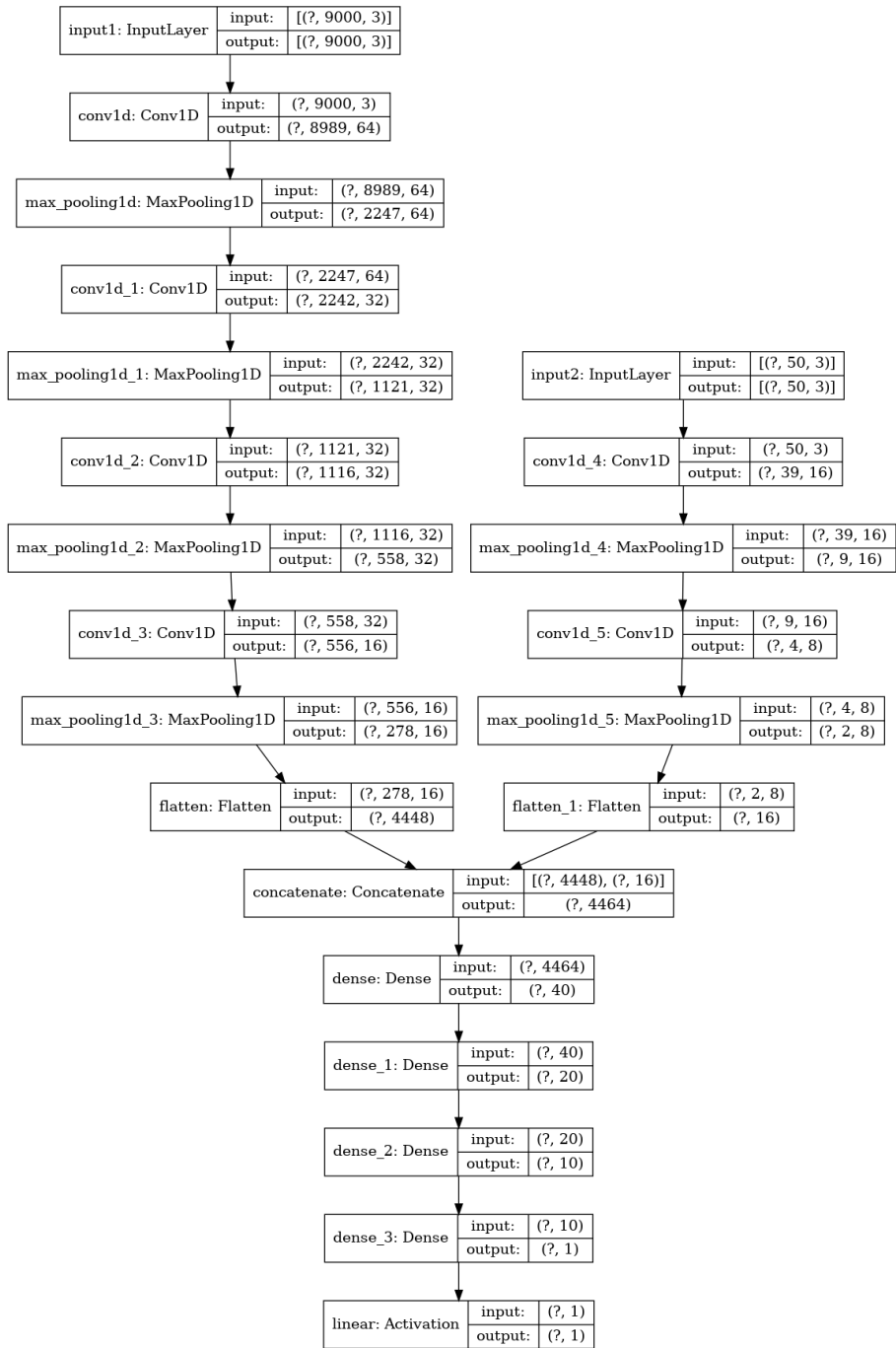
Figure 9: Architecture of Model 8.
