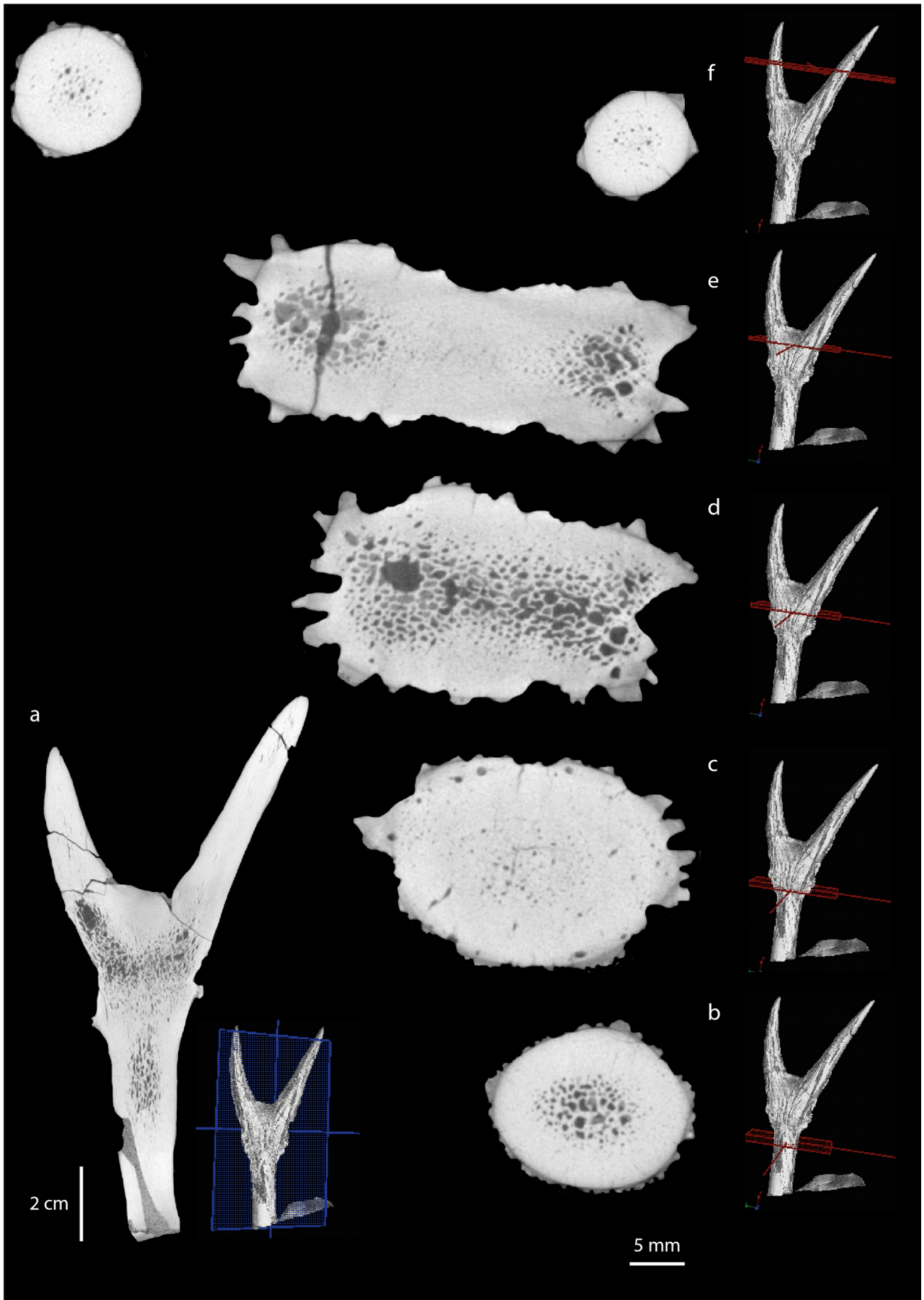
Online Resource 34: Radiographic sections of Heteroprox larteti , SMNS no number, Steinheim (Germany), Middle Miocene (MN7).
