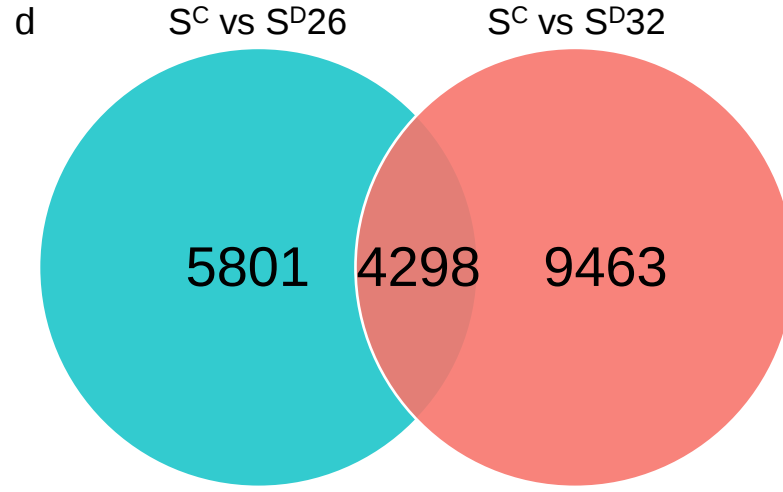
Fig. S2 DEGs induced by drought treatment at 26 DAP and 32 DAP for each isolate
