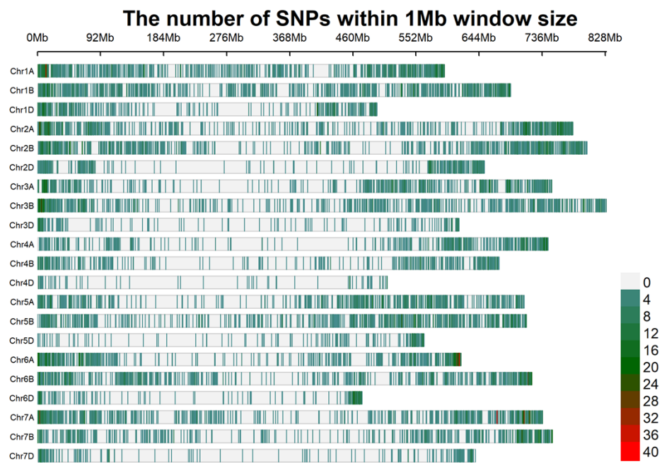
Additional file 5 Distribution of filtered SNPs on 21 wheat chromosomes. Colors indicate the number of SNPs within a 1 Mb interval.
