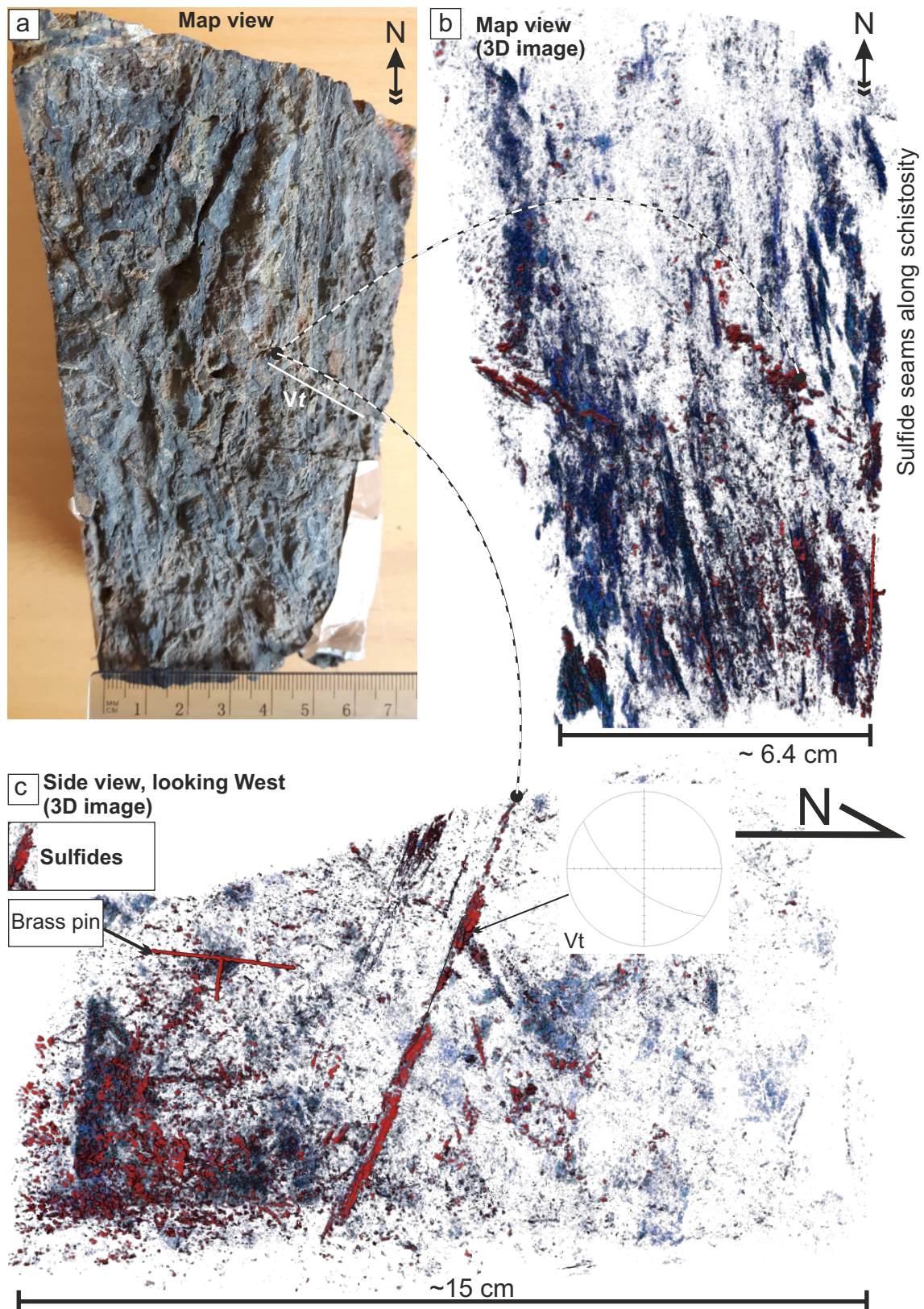
Online Resource 2 a Oriented sample Kittilä-01 showing the distribution of sulfides along S_R and Vt veins. b Three-dimensional (3-D) X-ray computed microtomography (XCT) image showing view from the top of the same sample. Voxel resolution is 65 \mu\text{m} . Rock matrix is rendered transparent. Sulfides are parallel to the main foliation ( S_R ) and also occur along the Vt veins. c Side view, looking toward the west and perpendicular to the S_R foliation of the same image as shown in b . Brass pin attached to the sample for strike-dip reference. Half arrow points up and North.
