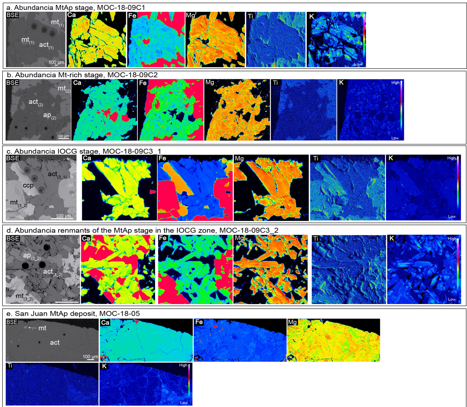
ESM Figure 3 EPMA X-ray maps of actinolite from samples in the Abundancia and San Juan deposits. a Sample MOC-18-09C1. b Sample MOC-18-09C2. c Sample MOC-18-09C3_1. d Sample MOC-18-09C3_2. e Sample MOC-18-05
