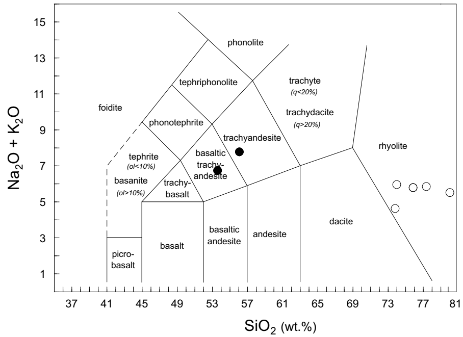
Fig. A31. Total alkalies versus \text{SiO}_2 plot for volcanic and pyroclastic rocks in the Roraima Supergroup.
