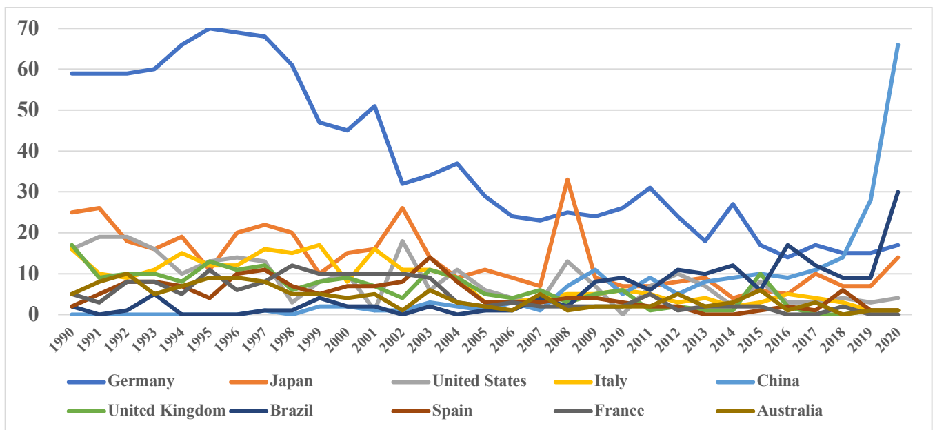
Fig. S14 Meta-Data: Publications by the TOP-10 contributing countries (1990-2020)
