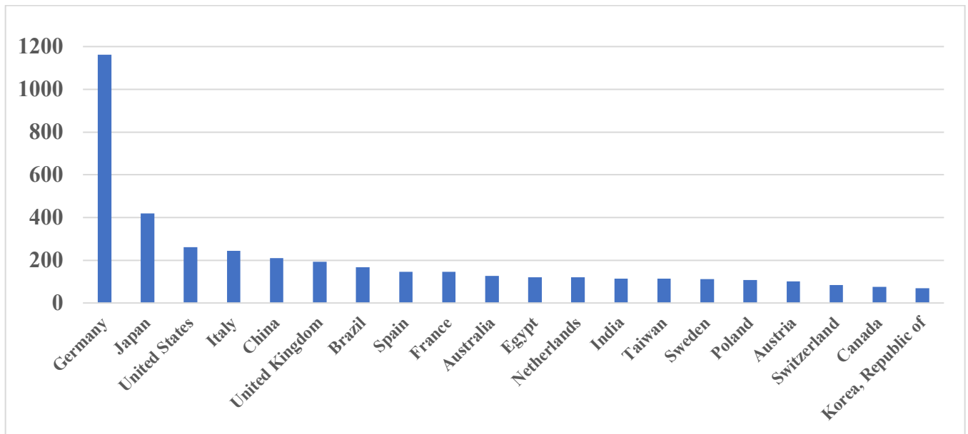
Fig. S13 Meta-data: Publications by the top-20 contributing countries (1990-2020)
