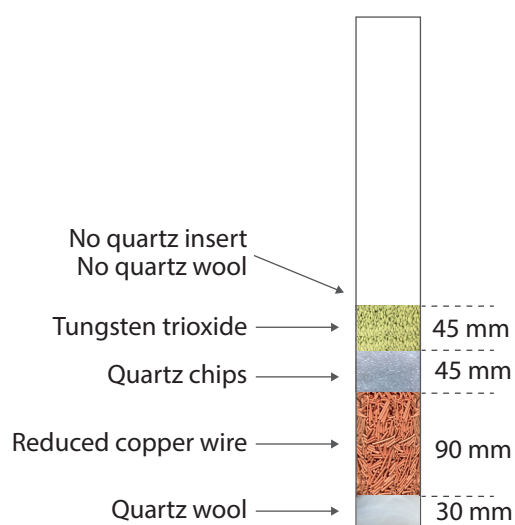
Fig. S1 Packing of reactor for sulfur isotope analysis by EA/IRMS.
