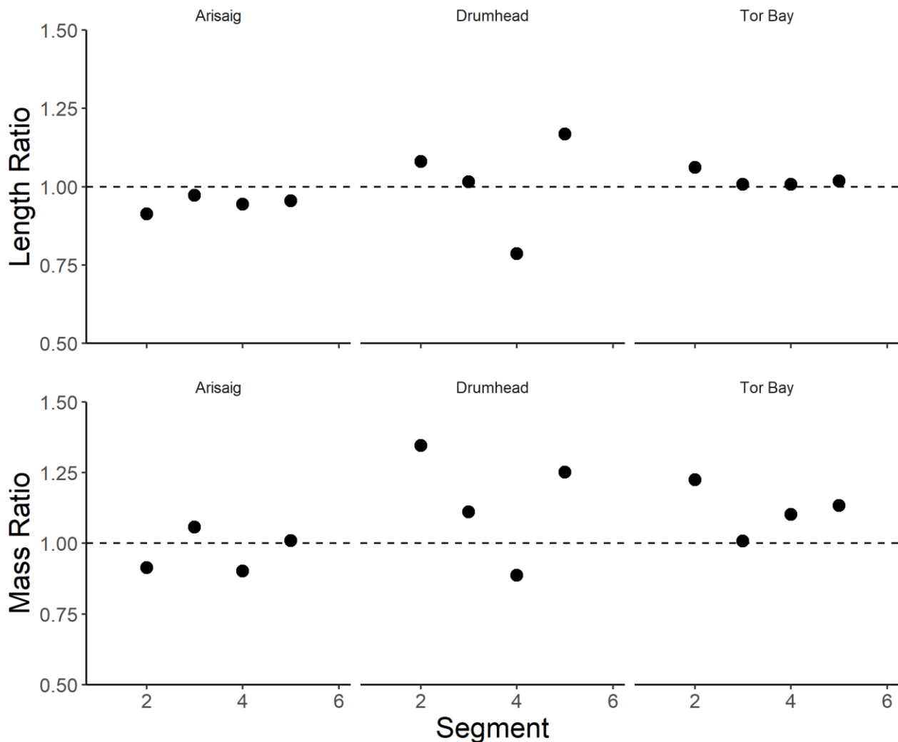
Fig. S1 Length and Mass ratios for Arisaig, Drumhead and Tor Bay in eastern Nova Scotia for the first 5 segments. Data were extracted from Figure 4 in Eckersley and Garbary (2007)
