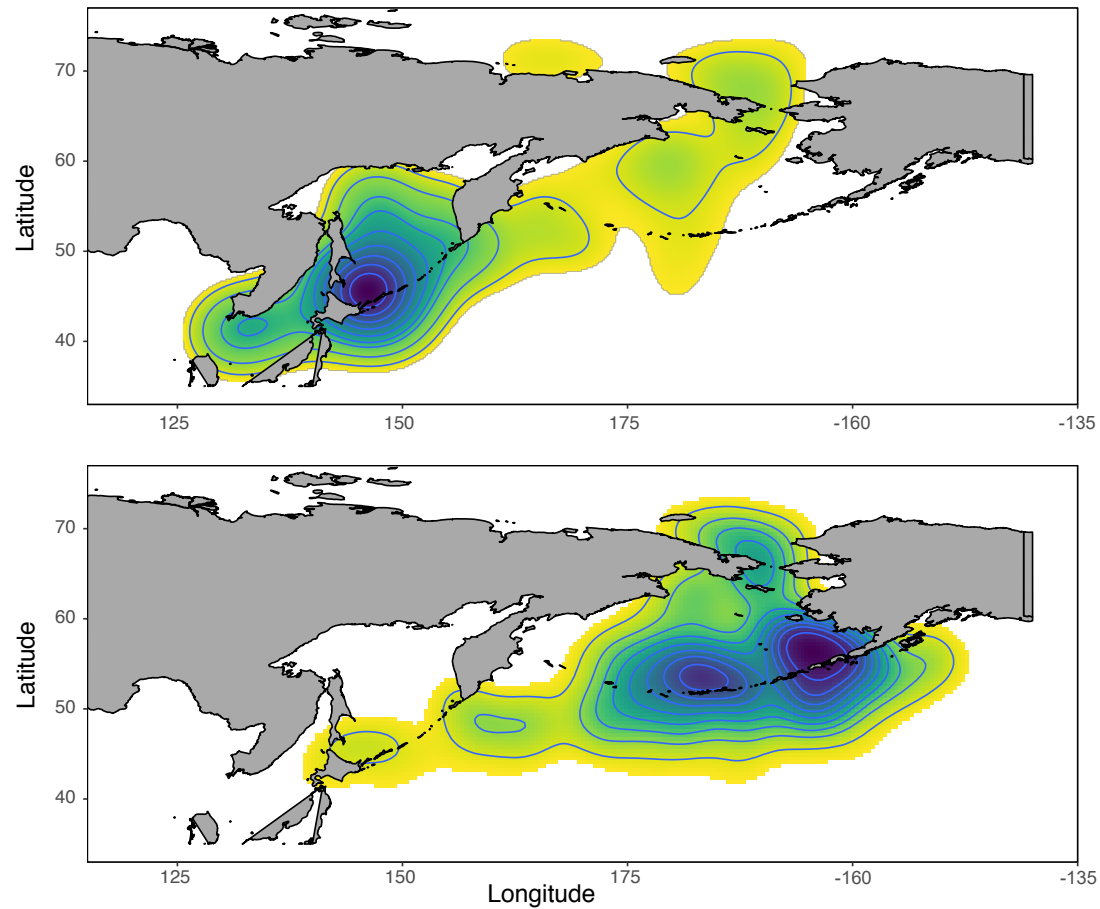
Fig. S1 The 95% KUD of cluster groups (Cluster 2 = Western group - Sea of Okhotsk/North Pacific, and Cluster 1 = Eastern group - southeast Bering Sea/North Pacific) of short-tailed shearwaters during the non-breeding season (May – October 2012 – 2016).
