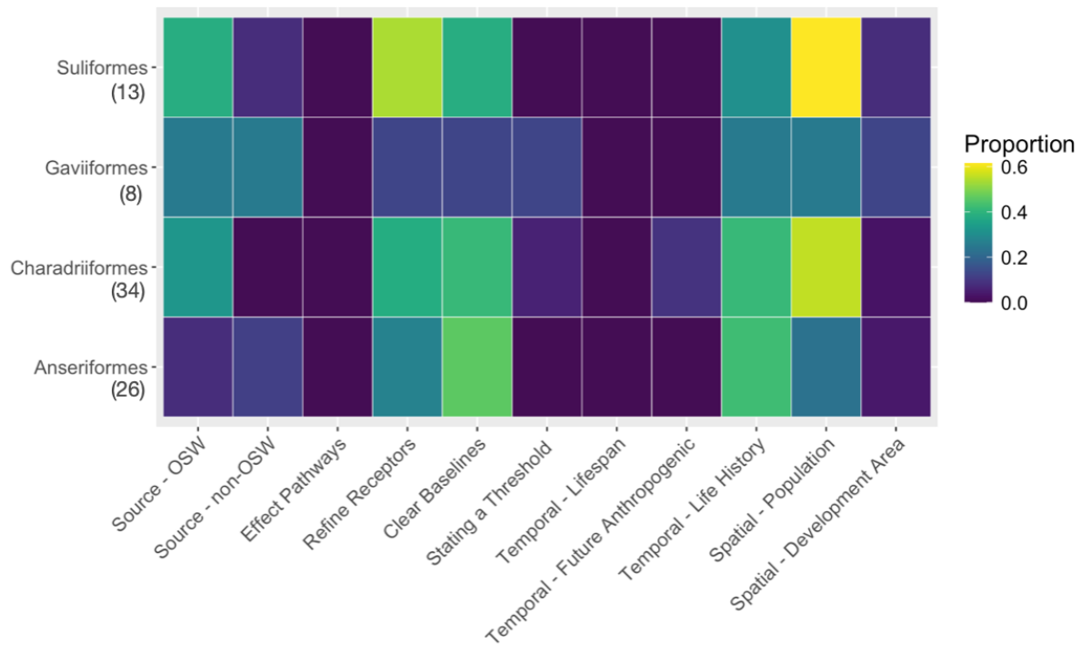
Supplementary Figure 2. Heat map showing the proportion of publications specific to each taxonomic order of marine waterbirds that included measurements for each category needed to assess the cumulative adverse effects of offshore wind installations on birds. Lighter colors (yellow) indicate that a measurement was addressed more often in the publications we reviewed, while darker colors indicate measures that were less frequently addressed. The number of publications in each group is shown in parentheses.
