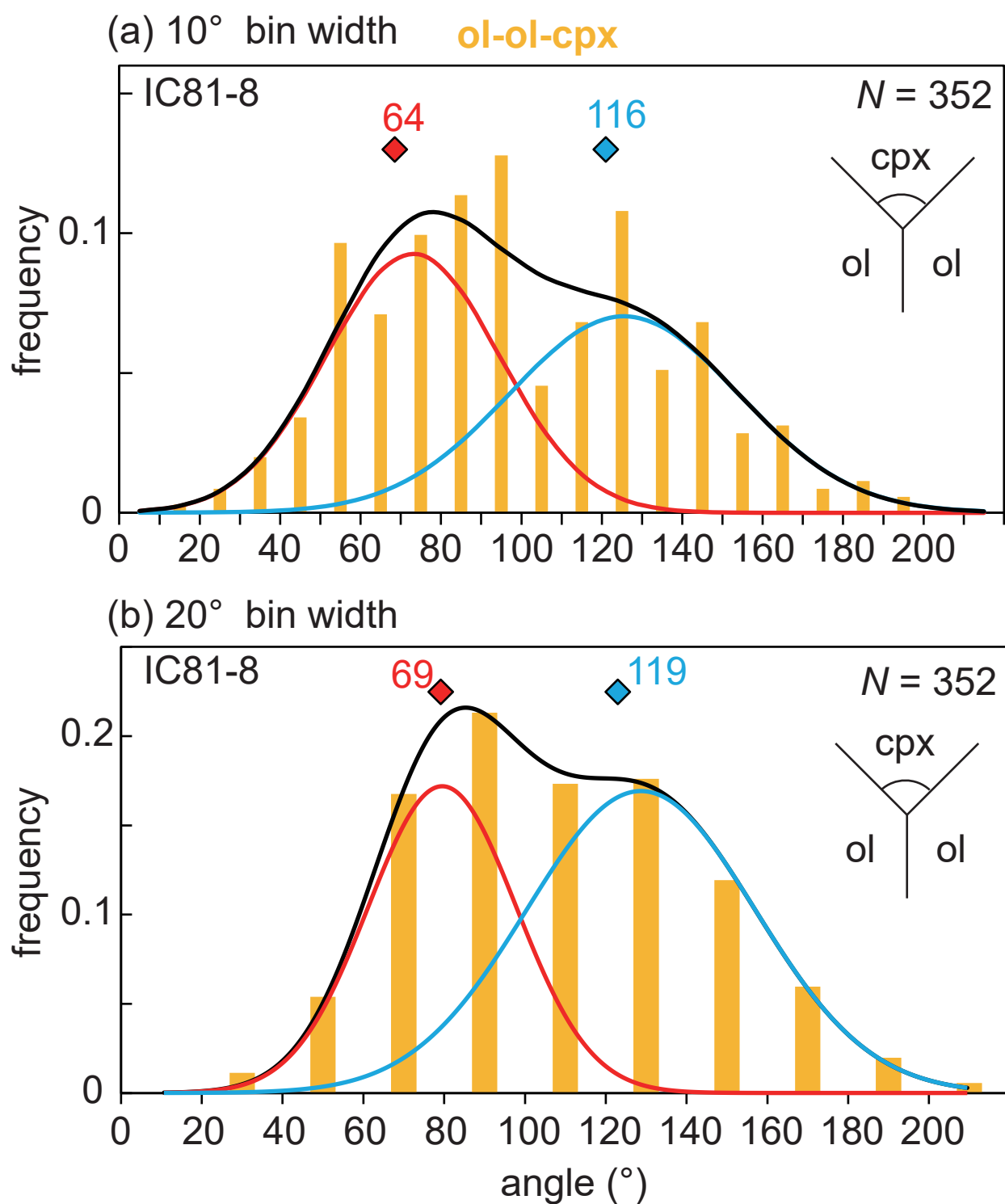
Fig. S1. Dihedral angles at ol-ol-cpx junctions in the Ichinomegata peridotite (sample IC81-8) with a bin width of (a) 10° and (b) 20°. The symbols and lines are as in Fig. 5. The numbers next to the diamond symbols indicate the mean of the corresponding normal distributions.
