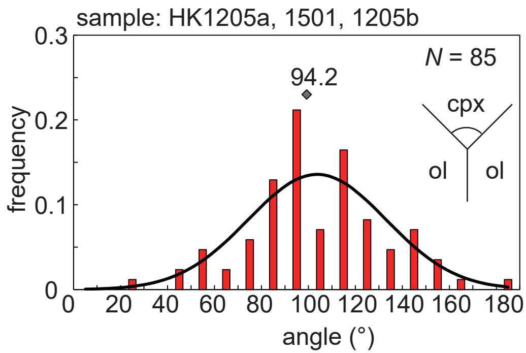
Fig. S2. Dihedral angles at ol–ol–cpx junctions located within one grain diameter of melt pockets in the Ichinomegata peridotite (HK1205a, HK1501, and HK1205b), in which melt pockets are abundant.
