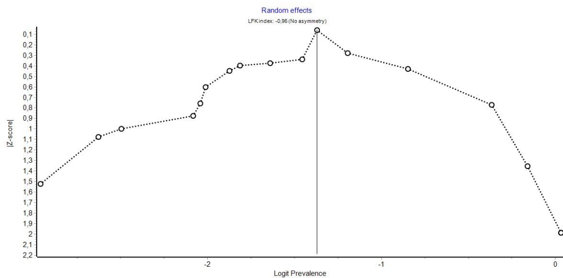
Supplementary figure 1 Doi plot with LFK index of patient-based evaluation
