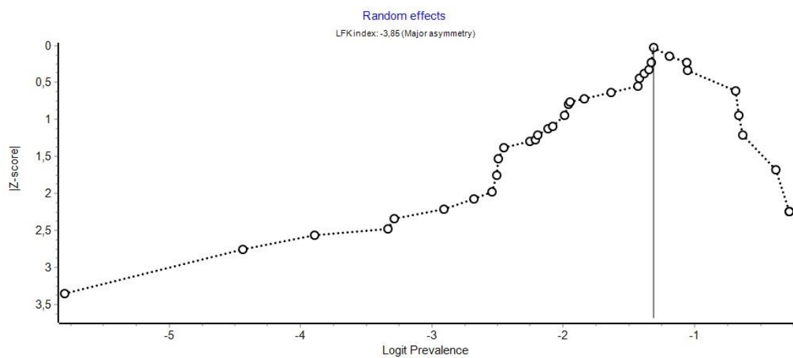
Supplementary figure 2 Doi plot with LFK index of feet-based evaluation
