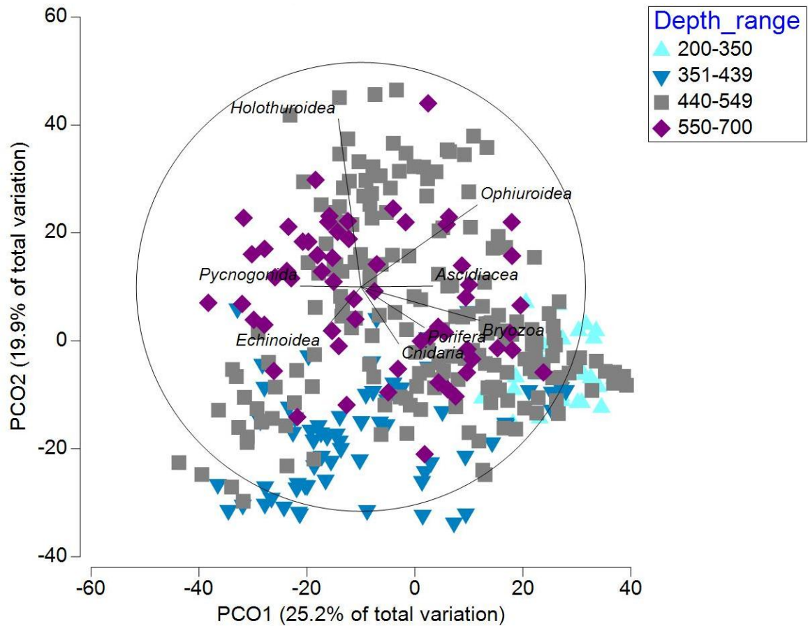
Online Resource 4 Principal Coordinate Analysis (PCO) plots of the NBP23-03 surveys showing variation in benthic community composition across different depth ranges highlighting faunal vectors with greater than 25% correlation with position of biotic ordination.
