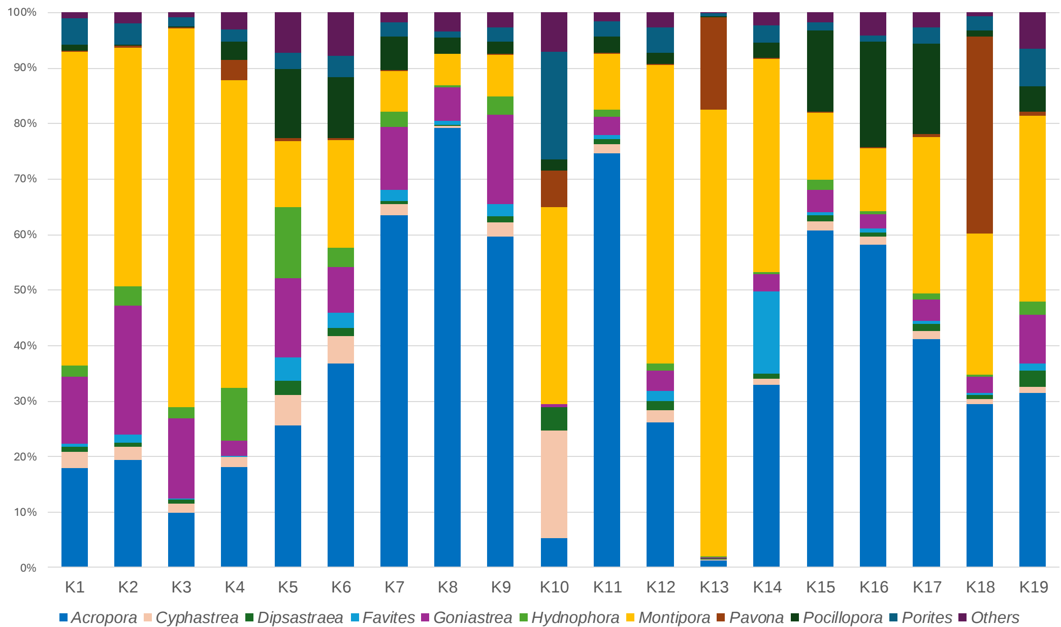
Fig. S1. Distributions and approximate proportions of scleractinian corals at each survey site in the Kerama Islands Names of scleractinian coral genera are shown below. See Fig. 1 for the locations of sites K1-K19).
