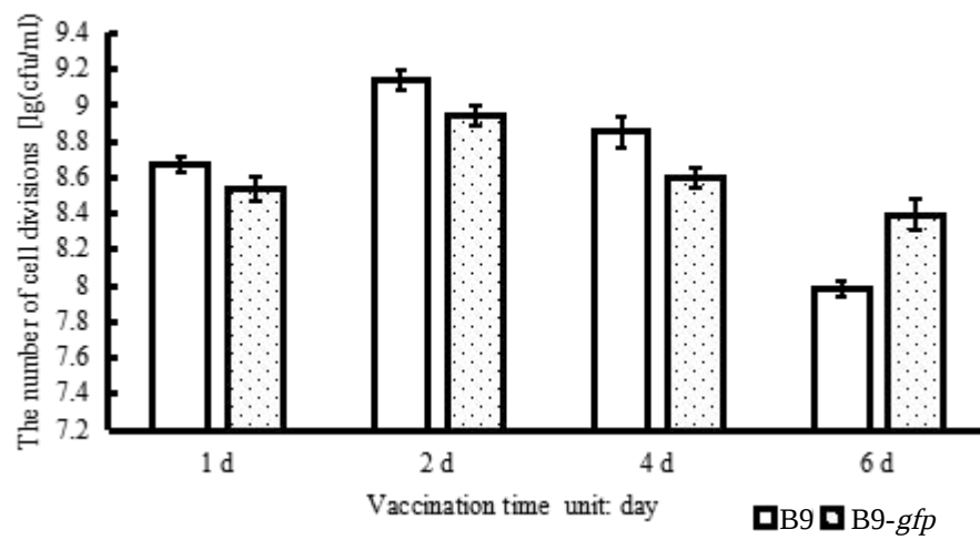
Figure S1 The growth rate of wild-type strain B9 and B9- gfp , and the data were presented as mean \pm standard error. The result shows that there was no difference in growth rates between the wild-type strain B9 and B9- gfp .
