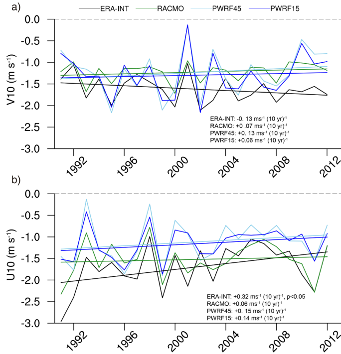
Fig. S7. Time series (1991–2012) of summer (DJF) (a) 10-m meridional wind and (b) 10-m zonal wind components averaged over a box covering Alexander Island in the central-southern windward coasts. The black line corresponds to ERA-Interim; green, light blue and dark blue lines are the simulations of RACMO, PWRF-45 and PWRF-15, respectively. Also included are the trend lines for each
