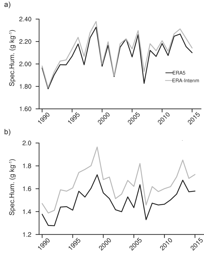
Fig. S2. Time series (1990–2015) of autumn (MAM) 850-hPa specific humidity averaged over the (a) windward and (b) leeward
