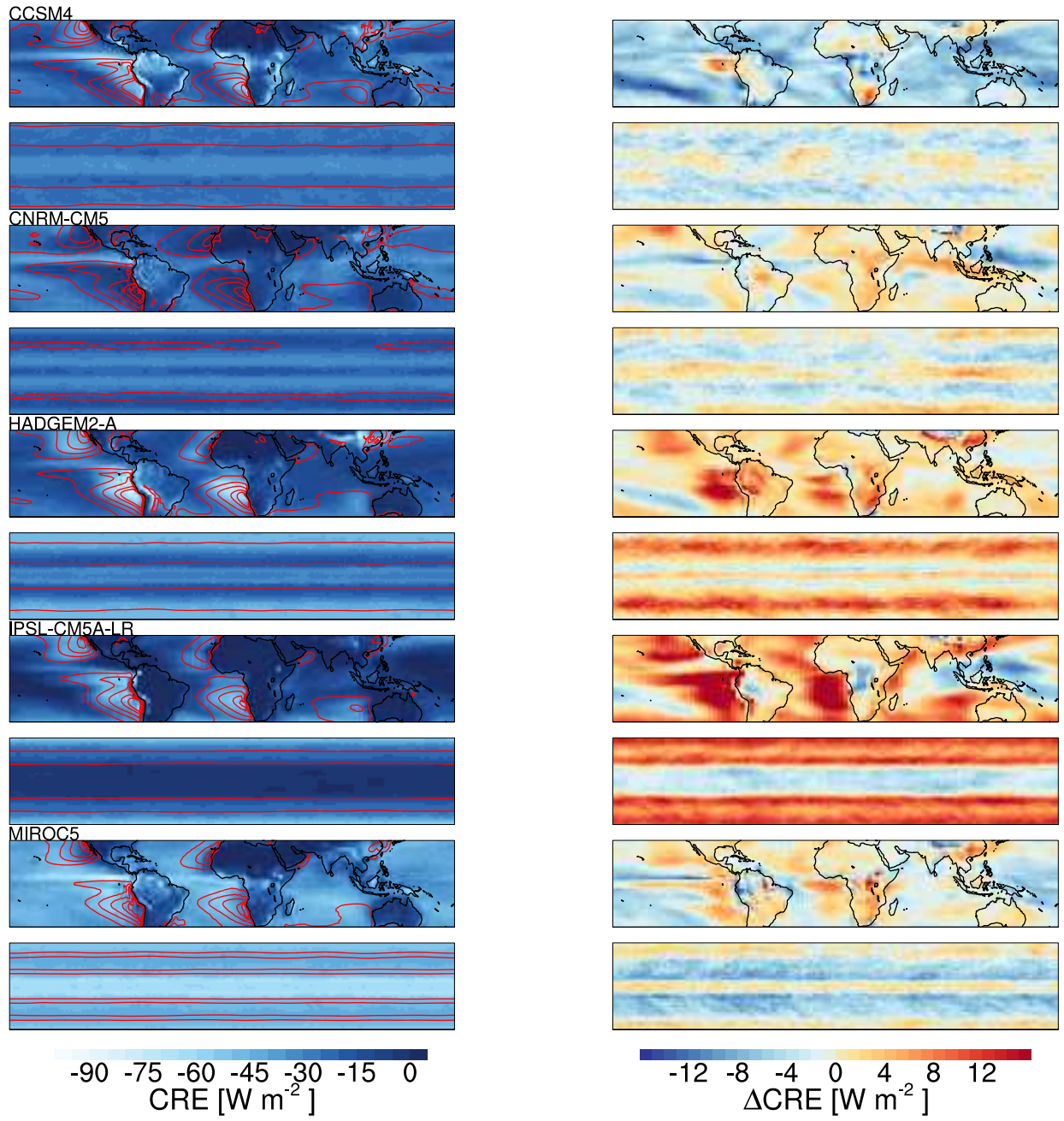
FIGURE 1. As in Fig. 12, but for the models with consistent \Delta\text{CRE} between AMIP and AQUA SST+4K experiments.
