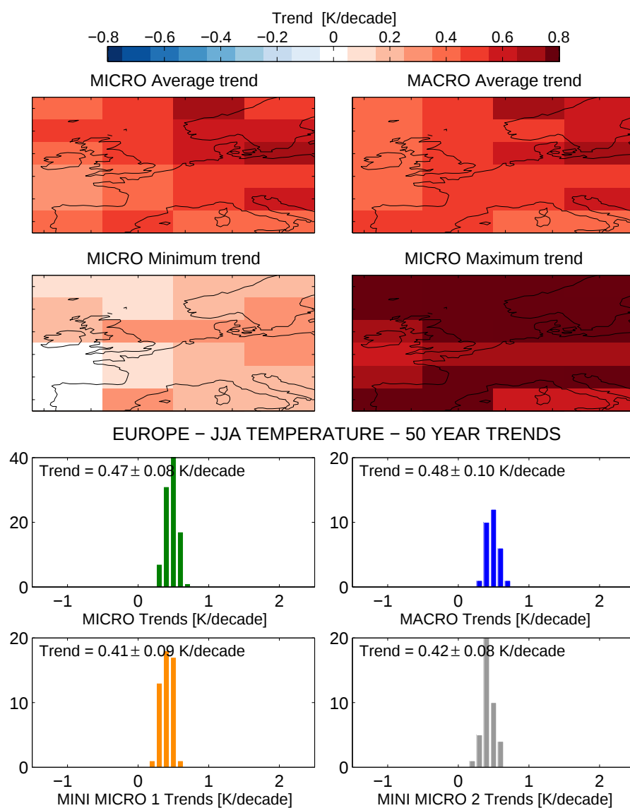
Fig. S3 As Figure S2 but for trends over the first 50 years. Note change of y-axis scales for the histograms.
