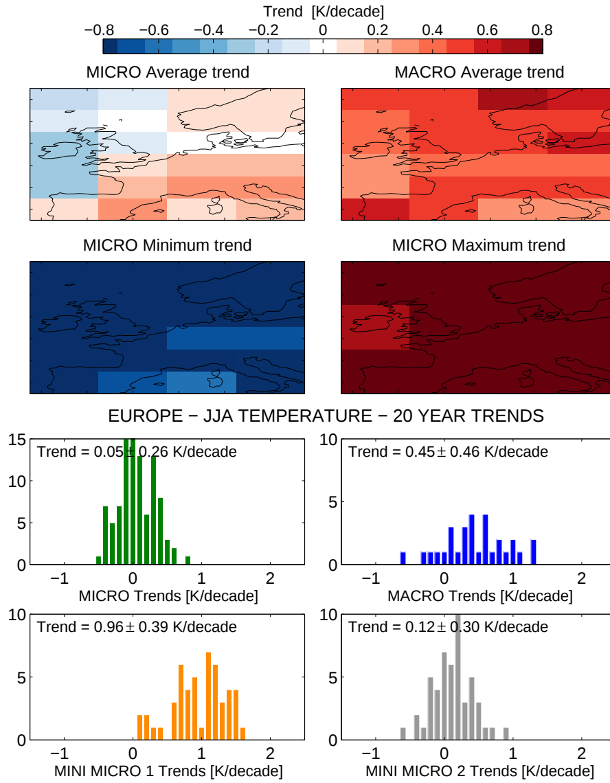
Fig. S2 Ensemble mean summer (JJA) trends over the first 20 years (top row) for the MICRO (left) and MACRO (right) ensembles, along with the maximum and minimum trend at any particular grid-point across the MICRO ensemble (second row). The distribution of trends for the domain average are shown in the bottom two rows for all four ensembles.
