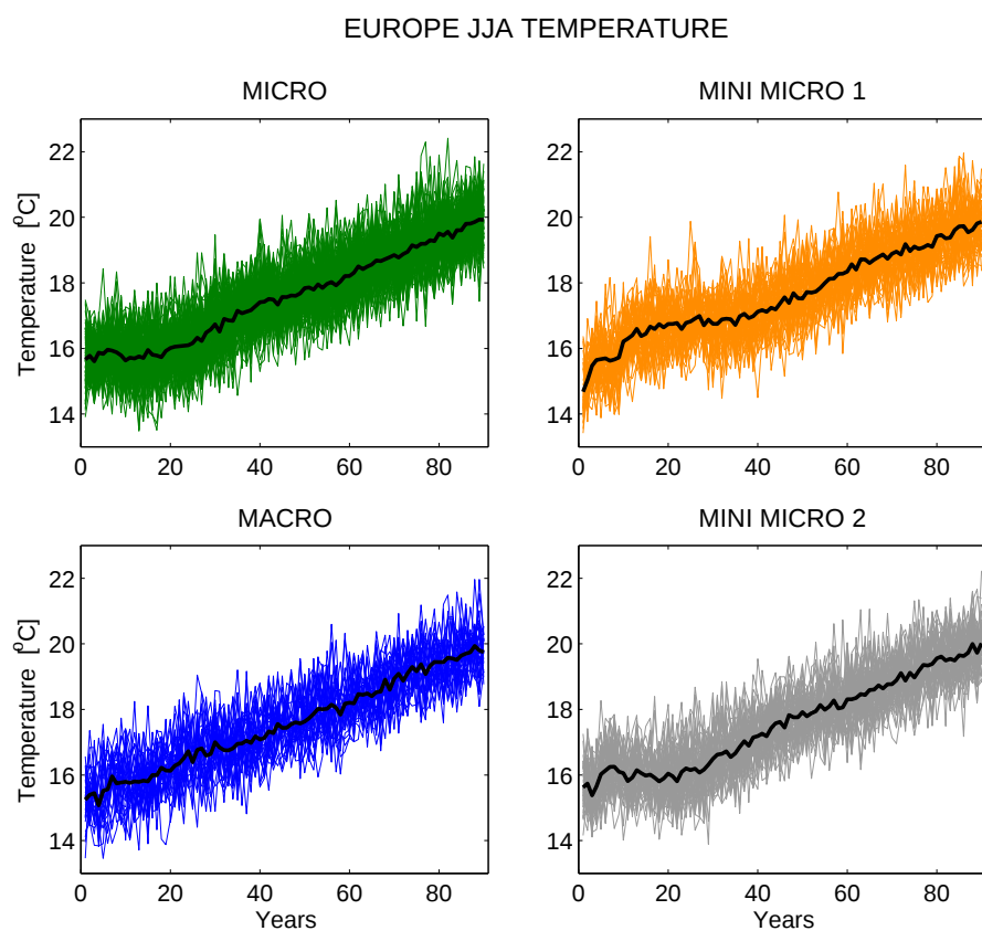
Fig. S1 Timeseries of Europe JJA temperatures in the various ensembles. The ensemble mean is shown in black.
