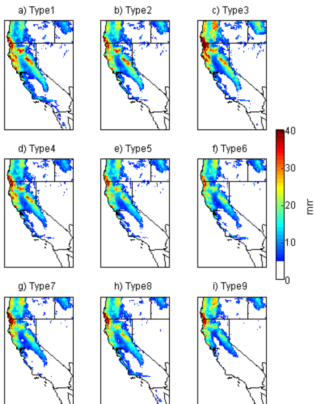
Figure S3. Average precipitation observed at the AR peak for each distinct type of AR.
