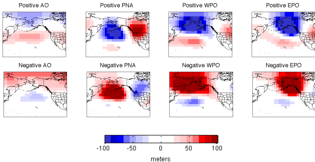
Figure S1. Composites of 500 mb geopotential height anomalies during Nov-Feb 1950-2013 when the North American Teleconnection indices were in the positive phase (top) and negative phase (bottom).
