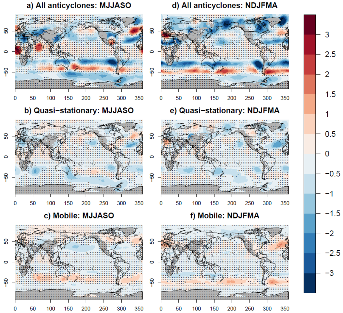
Figure S2. As in Figure 4, but with all anticyclone centres located at elevations over 1000m in ERA5 (regridded to a 1° resolution) removed prior to calculations. Areas with elevation above 100m are also shaded in grey.
