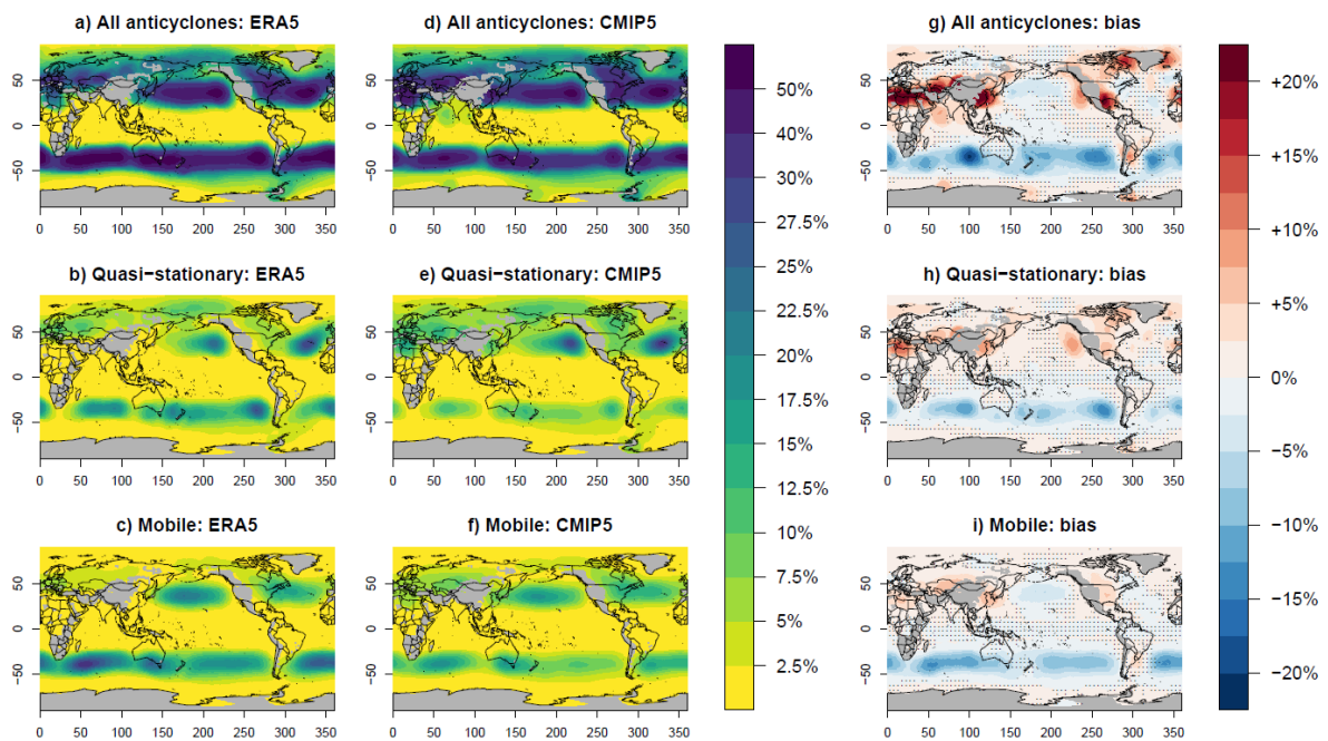
Figure S1. As in Figure 1, but with all anticyclone centres located at elevations over 1000m in ERA5 (regridded to a 1° resolution) removed prior to calculations. Areas with elevation above 100m are also shaded in grey.
