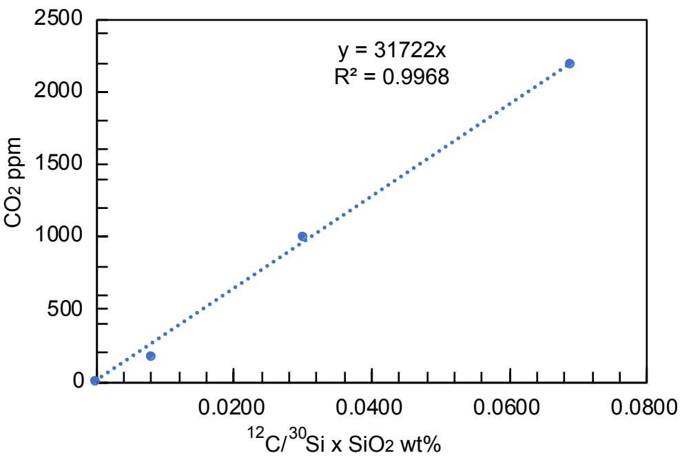
CO 2 calibration curve
