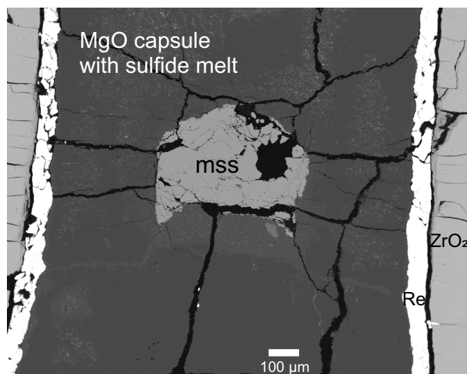
Figure 1. Backscatter-electron image of experiment E313, conducted at 14 GPa and 1355 °C showing the incipient melt trapped in the MgO capsule.
