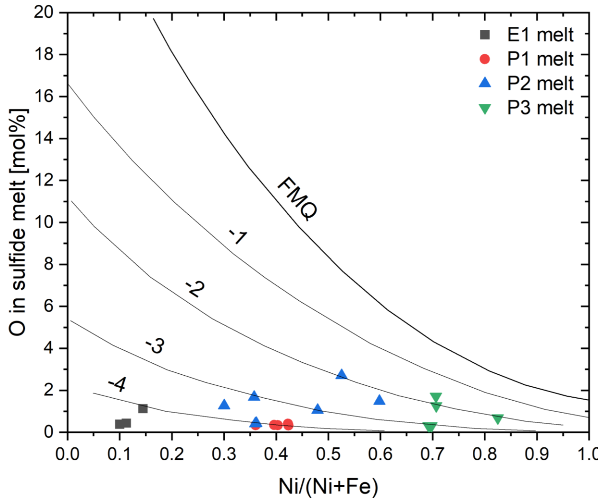
Figure 2: Oxygen concentration in sulfide melt vs. Ni/(Ni+Fe). The figure is redrawn from Zhang et al. (2018).
