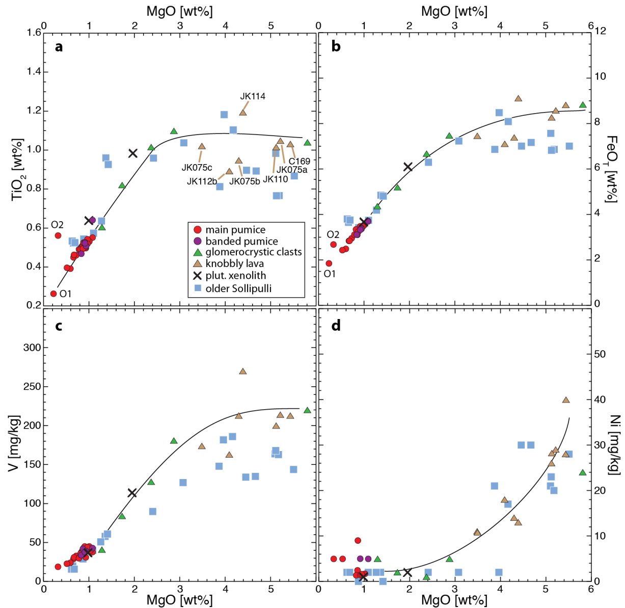
Fig. S5 MgO variation diagrams for (a) TiO 2 , (b) FeO as total iron, (c) V and (d) Ni bulk-rock concentrations of Alpehué and older Sollipulli (from Murphy, 1996) rocks. Note deviation of obsidian fragment O2 particularly in (a).
