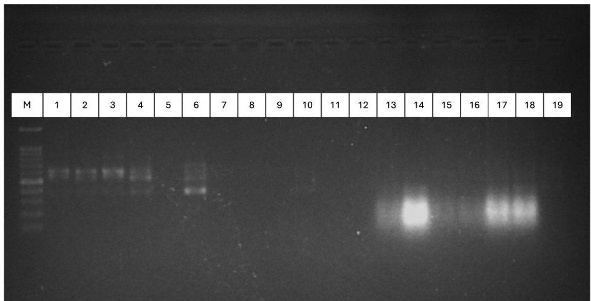
Fungal DNA visualized on a photographed gel electrophoresis
