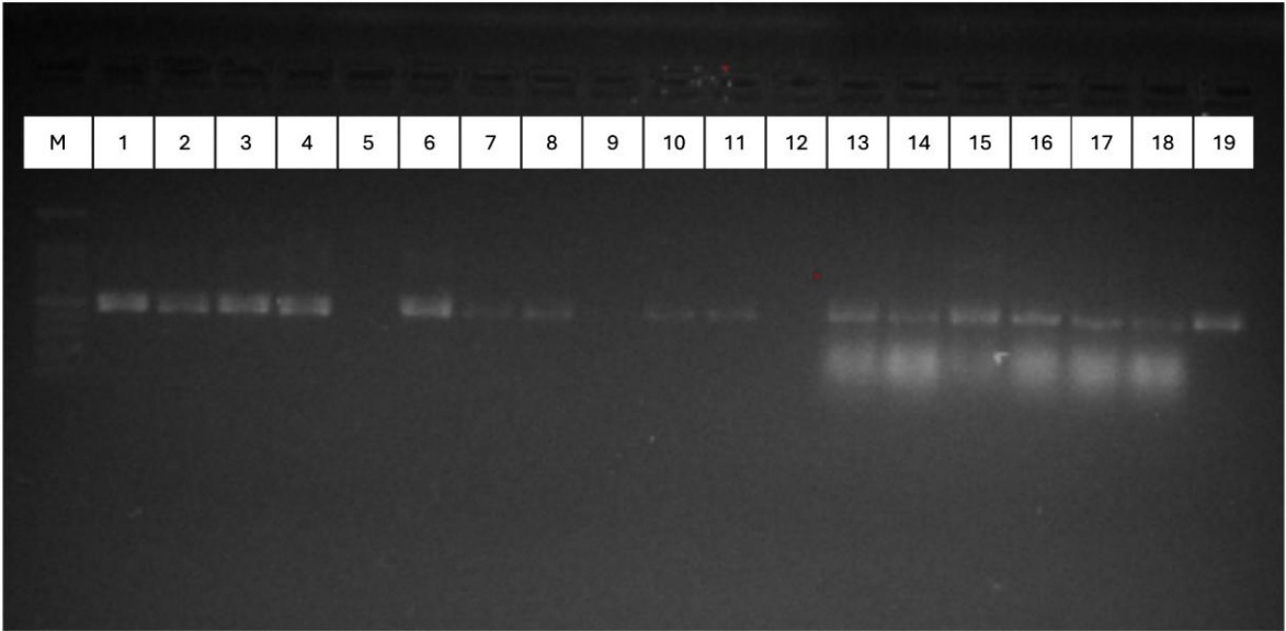
Bacterial DNA visualized on a photographed gel electrophoresis.
