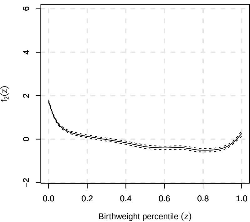
Main effect f_2(z)
