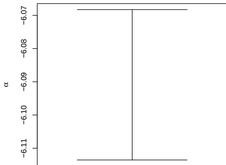
Intercept \alpha
