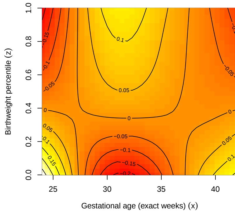
Interaction f_3(x, z)
