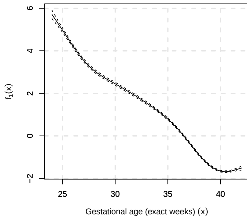
Main effect f_1(x)
