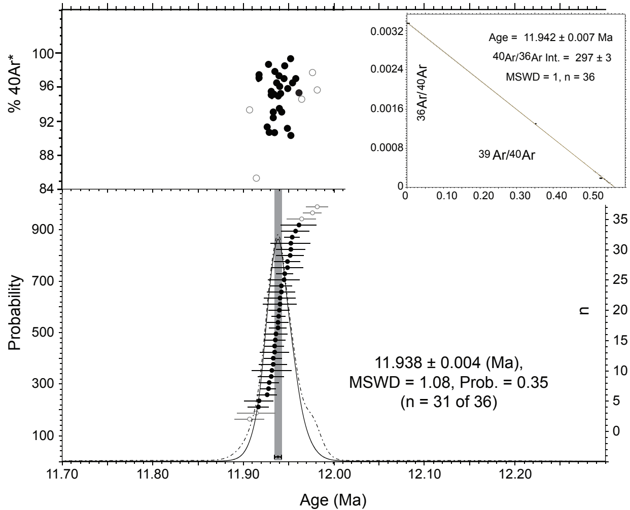
Figure S1a: Corral Creek Member (sample: BB-11.2-002; Lab-ID 31A - 2453)
