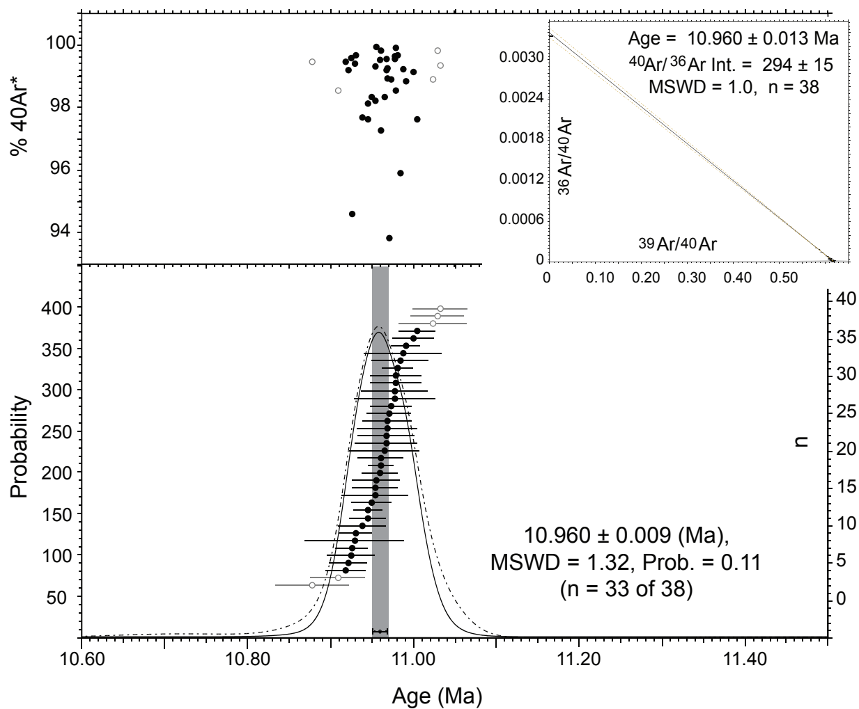
Figure S1d: Jackpot Member (sample: RG-10.1-007; Lab ID 2445)
