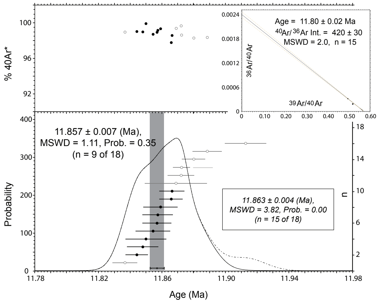
Figure S1b: Browns Bench Member (sample: RG-10.1-015; Lab-ID 31A - 2451)
