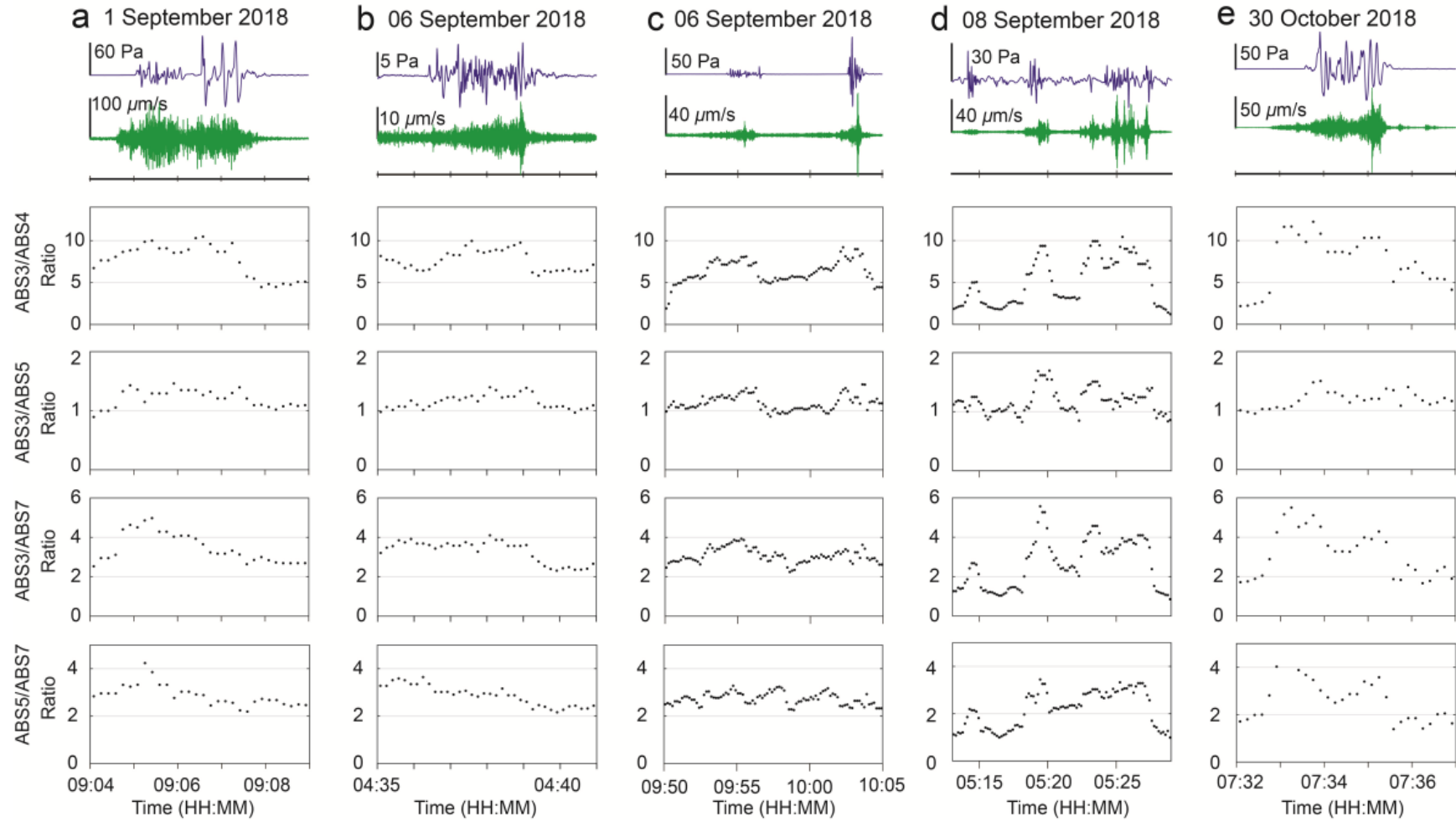
Fig. S4 The ratio variations for the five explosions on a 1 September 2018, b and c 6 September 2018, d 8 September 2018, and e 30 October 2018. Panel 1 shows acoustic (blue; ABA5) and seismic (green; ABS5) unfiltered waveforms (the same as Fig. 3), blow panels indicate ratio variations with time using ABS3/ABS4, ABS3/ABS5, ABS3/ABS7, and ABS5/ABS7.
