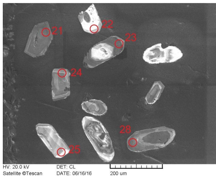
Battonya–Pusztaföldvár Basement Ridge (BATR/2 sample)
