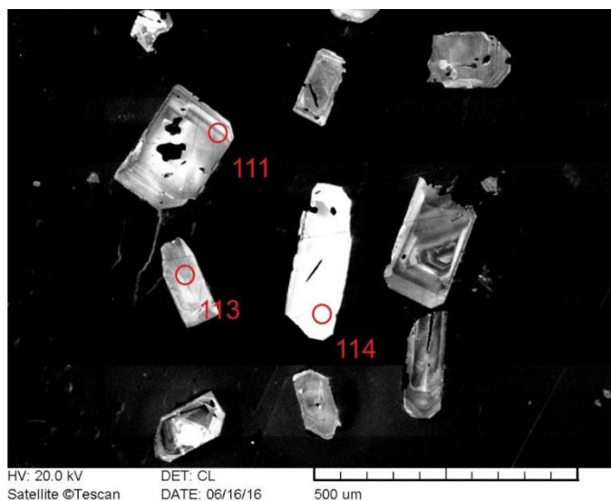
Battonya–Pusztaföldvár Basement Ridge (BATR/2 sample)
