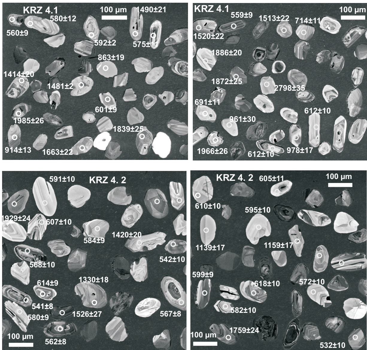
ESM 11 East European Platform, examples of zircons of the revealed age groups
