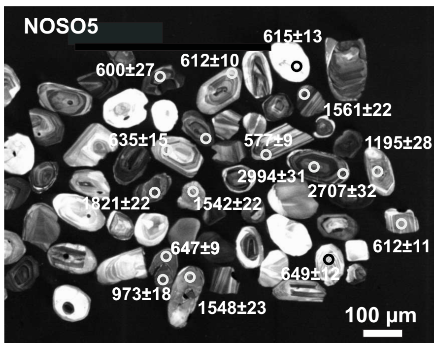
ESM 5 Małopolska Block, examples of zircons of the revealed age groups in Tremadocian sandstones
