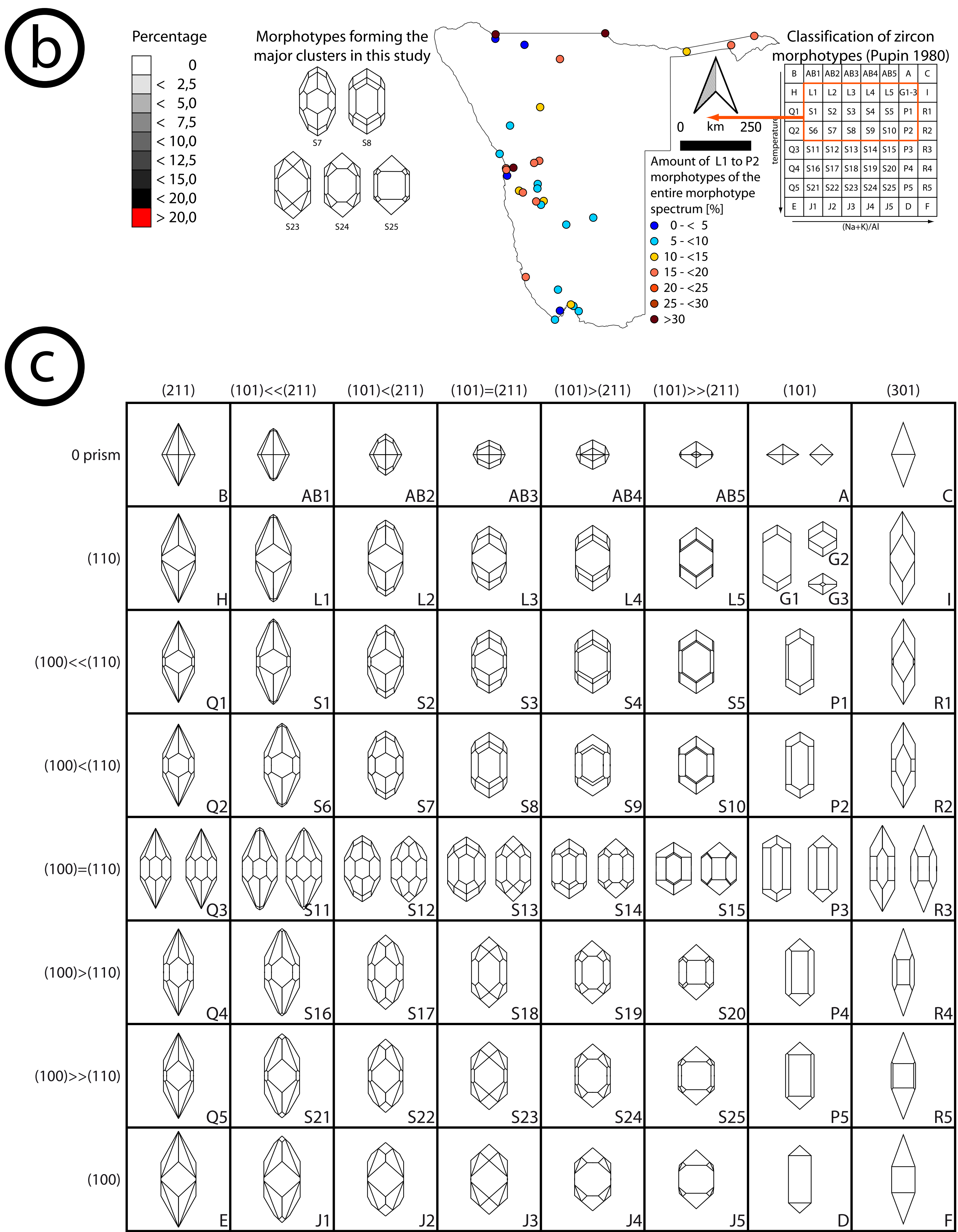
Fig.S1: a) Distribution of zircon morphotypes per sample for all samples of this study and Gärtner et al. (2014) according to Pupin (1980). b) Spatial distribution of L1 to P2 morphotypes in the samples shown in a). c) Morphotypes of zircon according to Pupin (1980).
