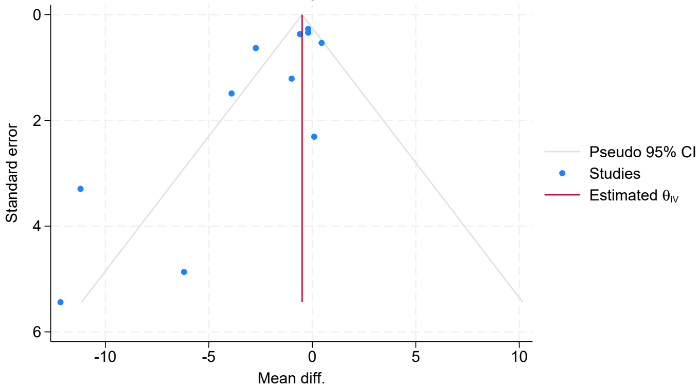
Funnel plot
