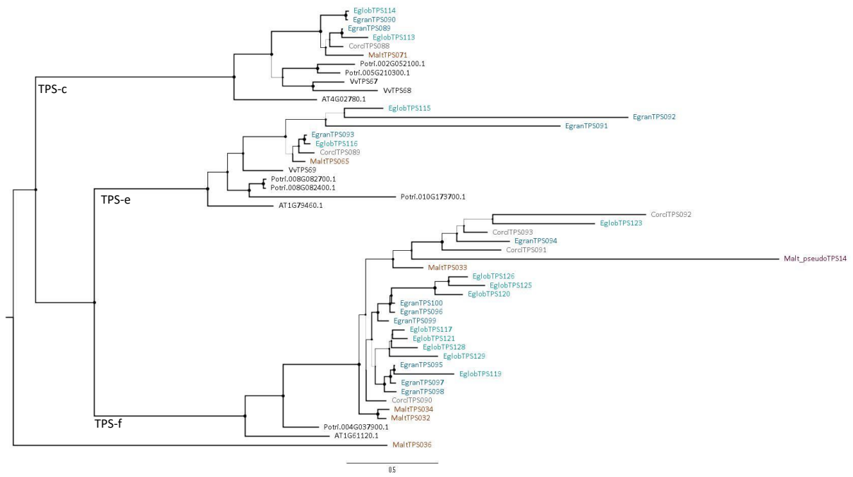
Online Resource 7 c Phylogenetic tree representing the TPS-c, TPS-e, and TPS-f subfamilies, including M. alternifolia pseudogenes. MaltTPS036 (TPS-b) was used as outgroup.
