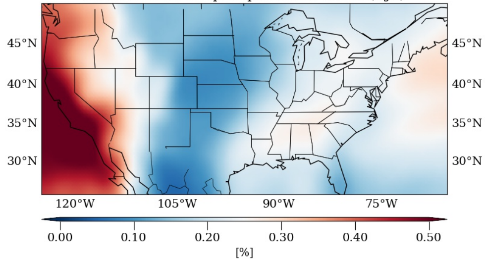
Fraction of annual precipitation in winter (DJF)
