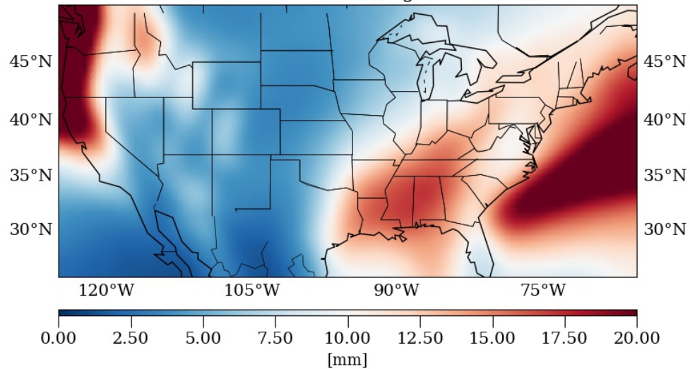
Mean winter rainfall during 1980 to 2020
