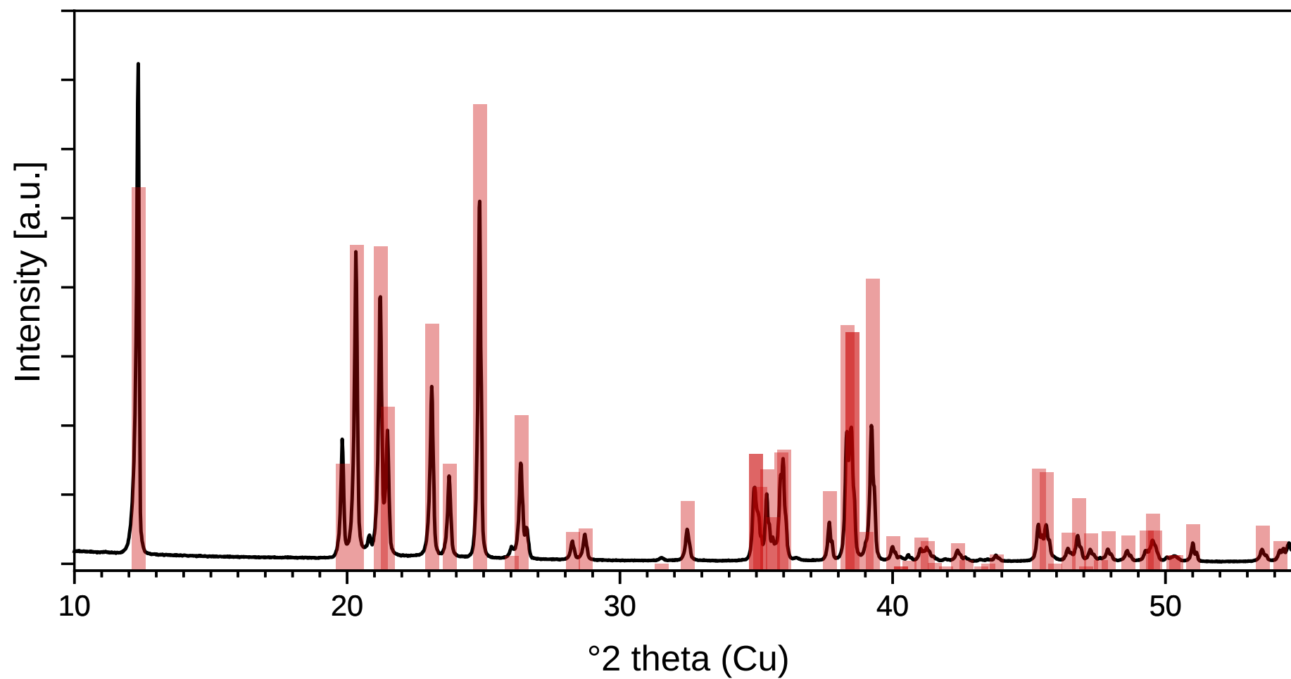
Fig. S2 Diffraction pattern of kaolinite from inside an agate geode of Börtewitz (black lines; background corrected) and the theoretical line positions (red) of kaolinite (PDF 04-013-2815, ICDD)
