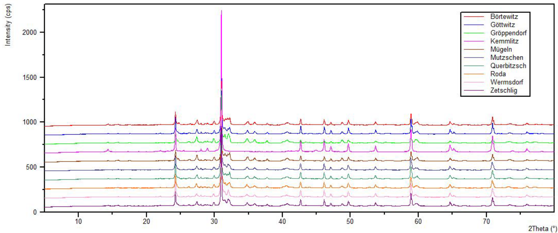
Fig. S1 Diffraction patterns (background corrected) of a porphyritic rhyolite from Zetschlig and lithophysae from different locations of the Kemmlitz rhyolite (see inset)
