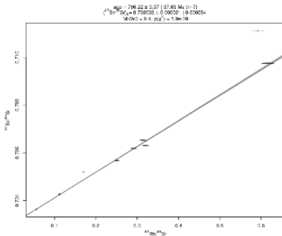
ESM3 Fig. Rb-Sr isotope errorchron of bulk-rock kimberlite samples from Camp Alpha. The size of the ellipses indicates the uncertainties of individual analyses; colourless ellipses are outliers not included in the regression. MSWD - Mean Square Weighted Deviation.
