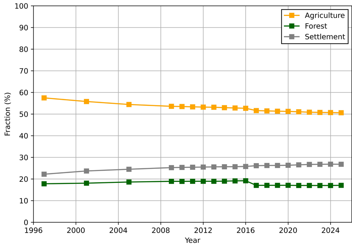
Figure S2. Development of the land use in the Viersen district. Data from Federal Statistical Office of Germany, available from https://www.regionalstatistik.de/genesis/online/logon (last access: 13.11.2025)
