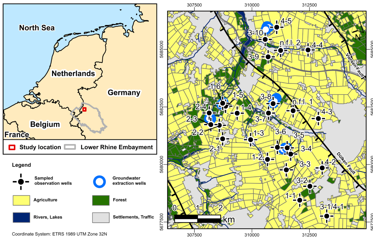
Figure S1. Map displaying the land use in the study area. Land use based on the current digital landscape model of North-Rhine Westphalia, available from https://www.bezreg-koeln.nrw.de/geobasis-nrw/produkte-und-dienste/landschaftsmodelle/aktuelle-landschaftsmodelle/digitales-basis (last access: 13.11.2025)
