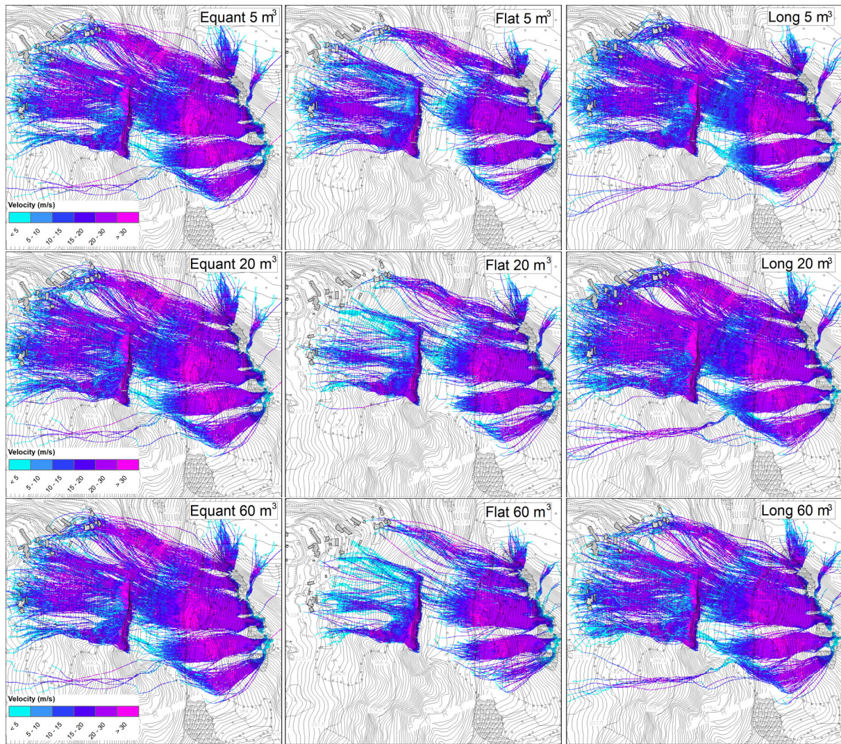
Trajectory maps with velocity ( \text{m s}^{-1} ) displayed along the rockfall paths for the nine scenarios.
