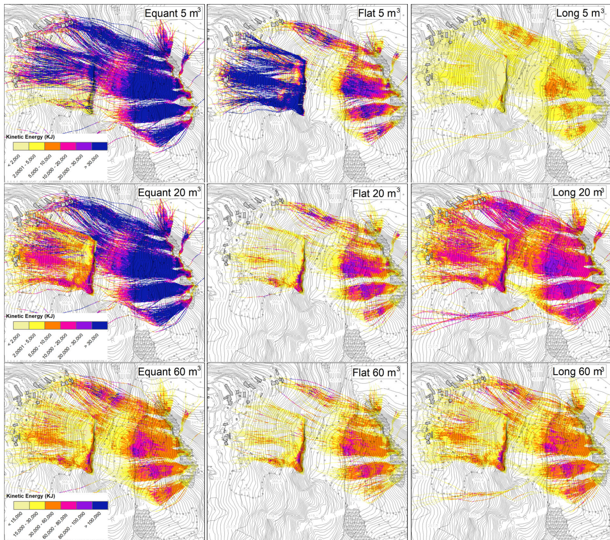
Trajectory maps with Kinetic Energy (KJ) displayed along the rockfall paths for the nine scenarios.
