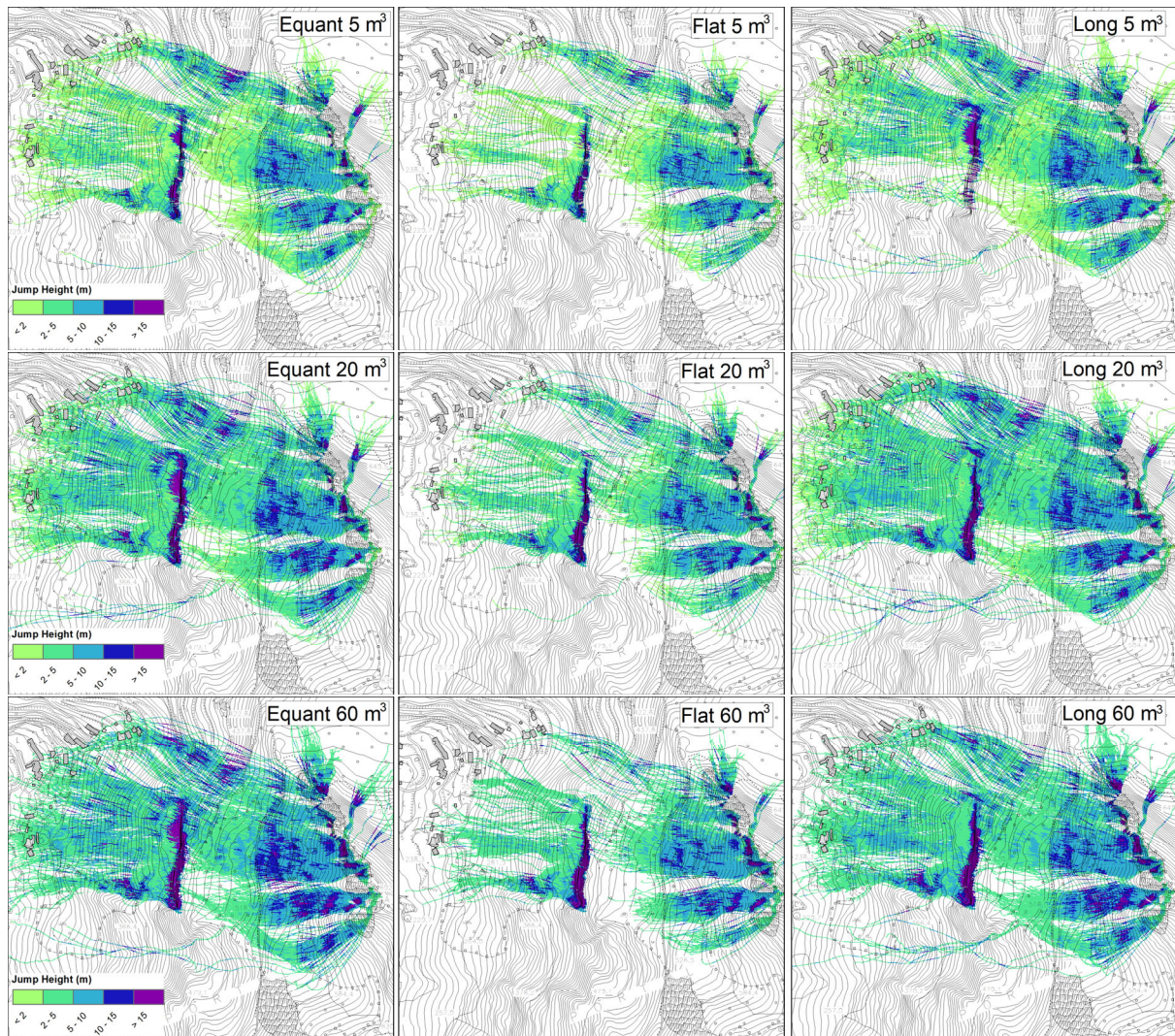
Trajectory maps with jump height (m) displayed along the rockfall paths for the nine scenarios.
