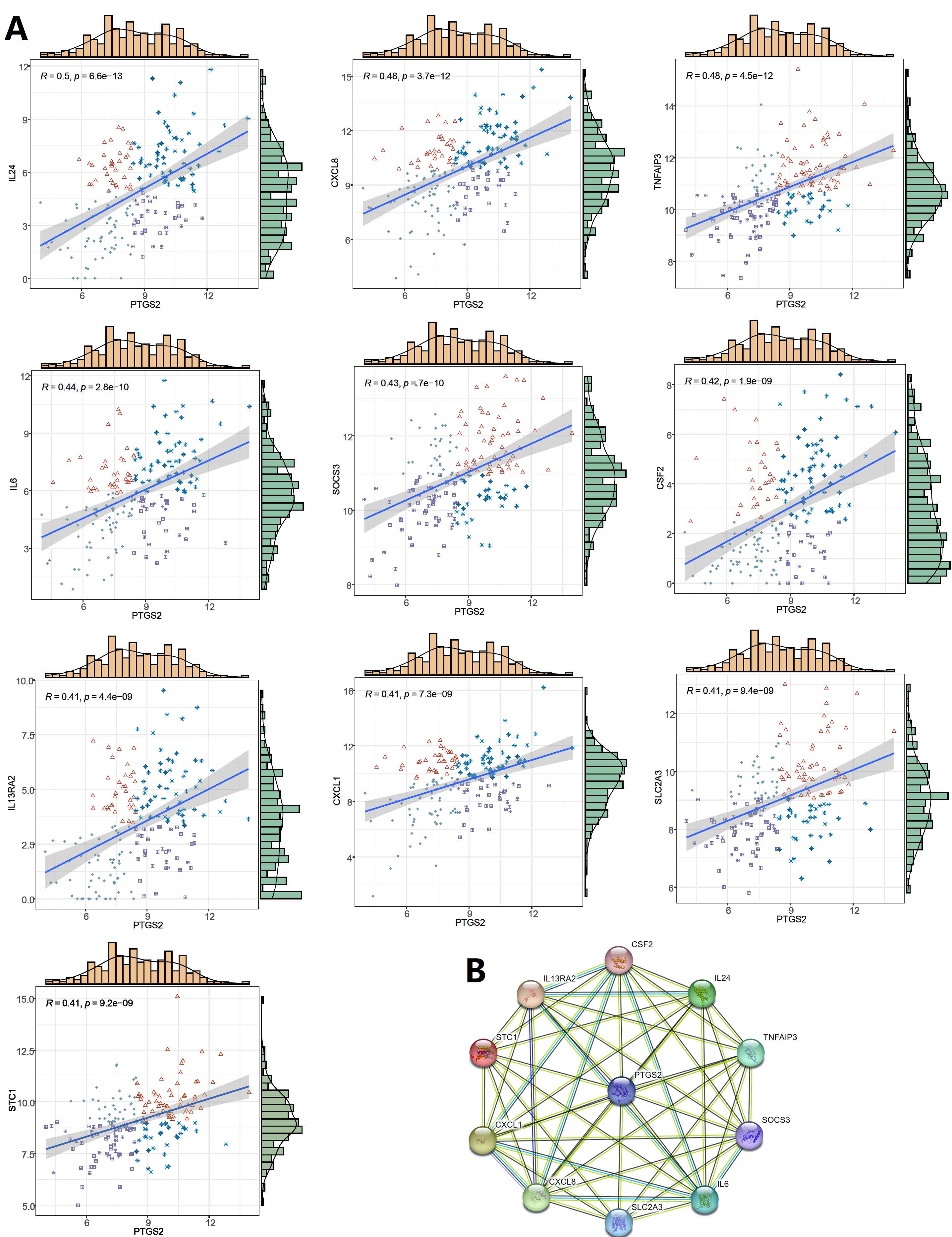
Figure S1. Top 10 genes most significantly correlated with COX-2 expression
