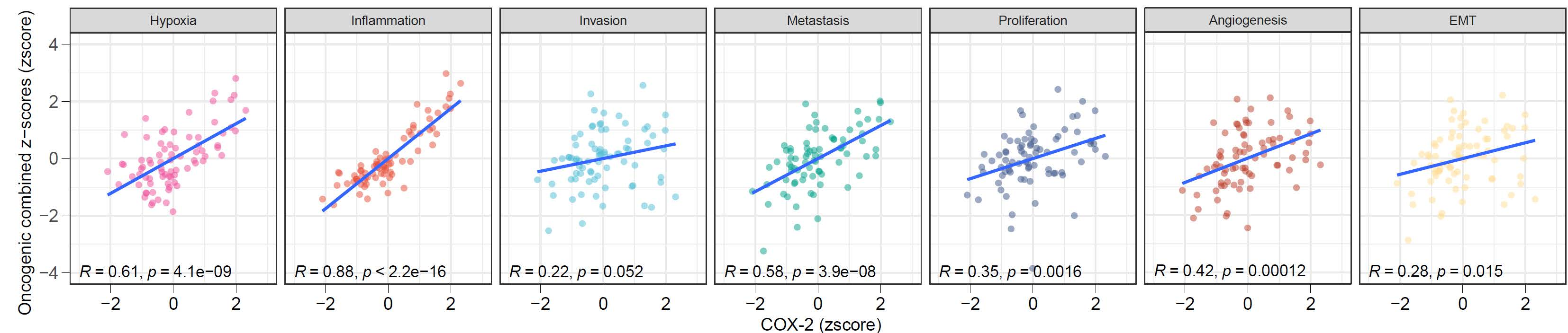
Figure S6. Correlation analysis of z-scores between COX-2 expression and various cancer-related processes in esophageal cancer in external datasets
