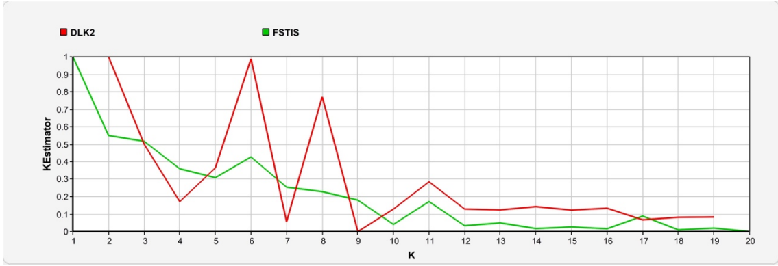
Fig S1. The estimated log-likelihood (DLK2) and FST/FIS values for the most suitable value of K in PopCluster analysis.
