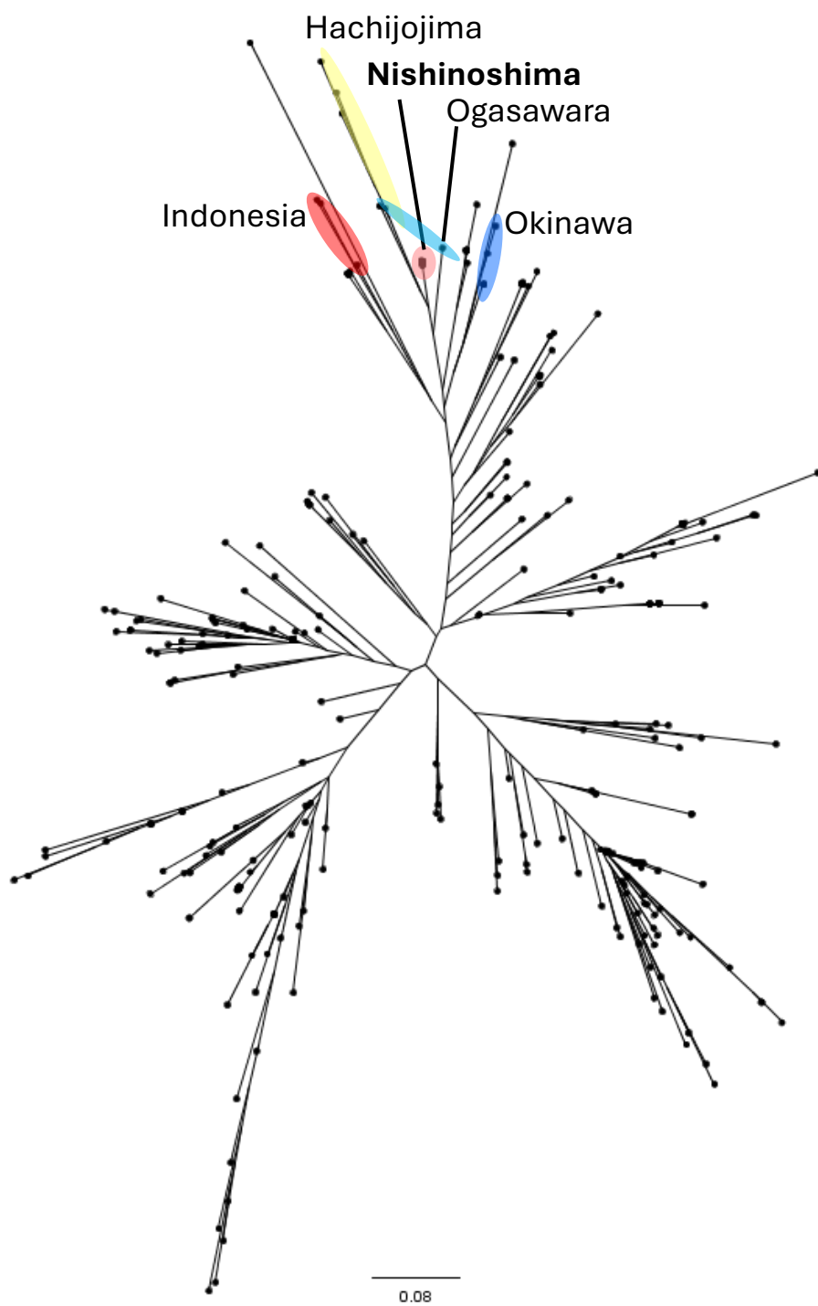
Fig. S3. The phylogenetic tree at individual level in Eleusine indica .
