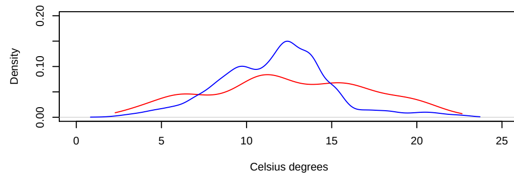
Spring temperature (Tmaxspring)
