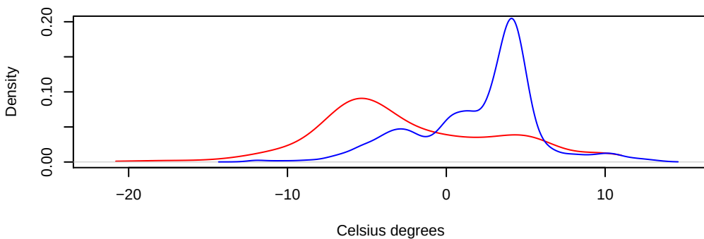
Winter temperature (bio11)
