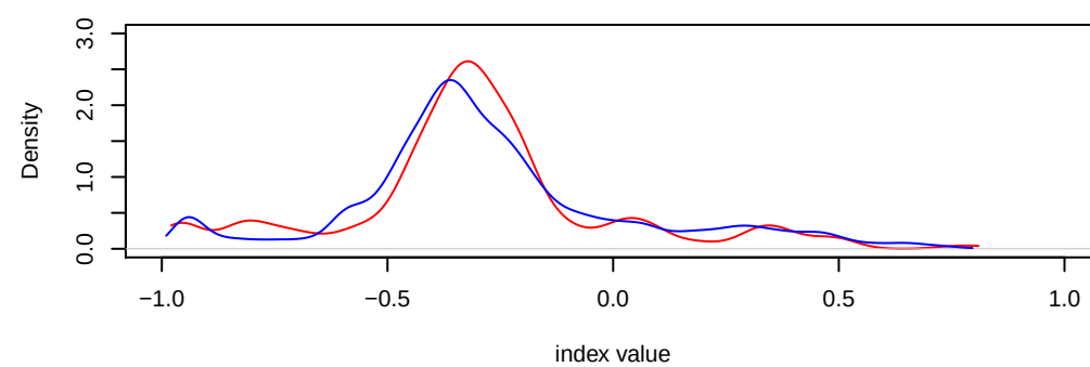
Climatic moisture index in summer (cmi_summer)
