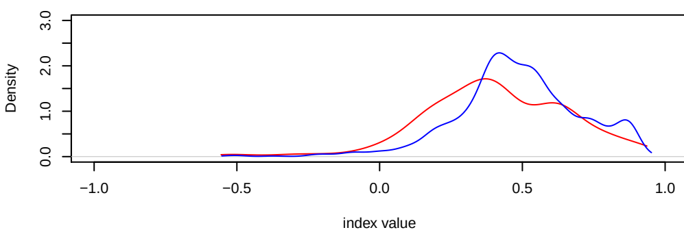
Climatic moisture index from fall to spring (cmi_8_coldest months)
