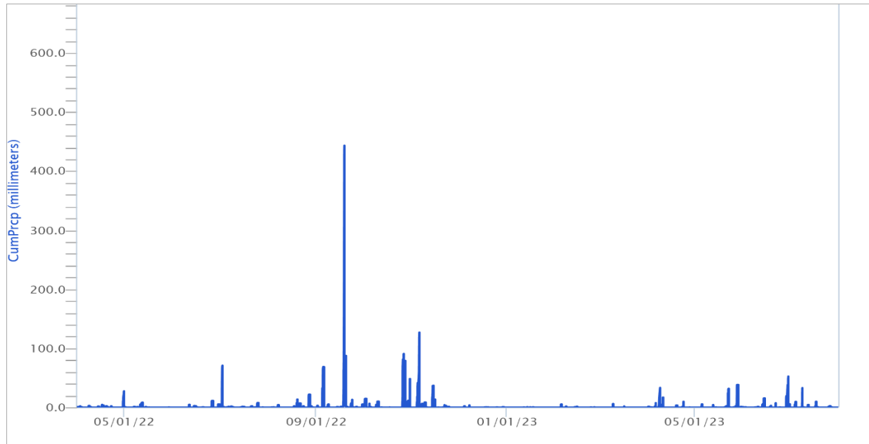
Fig. 1 Graph of cumulative precipitation (millimeters) in Jobos Bay during the study period (April 2022-July 2023).
