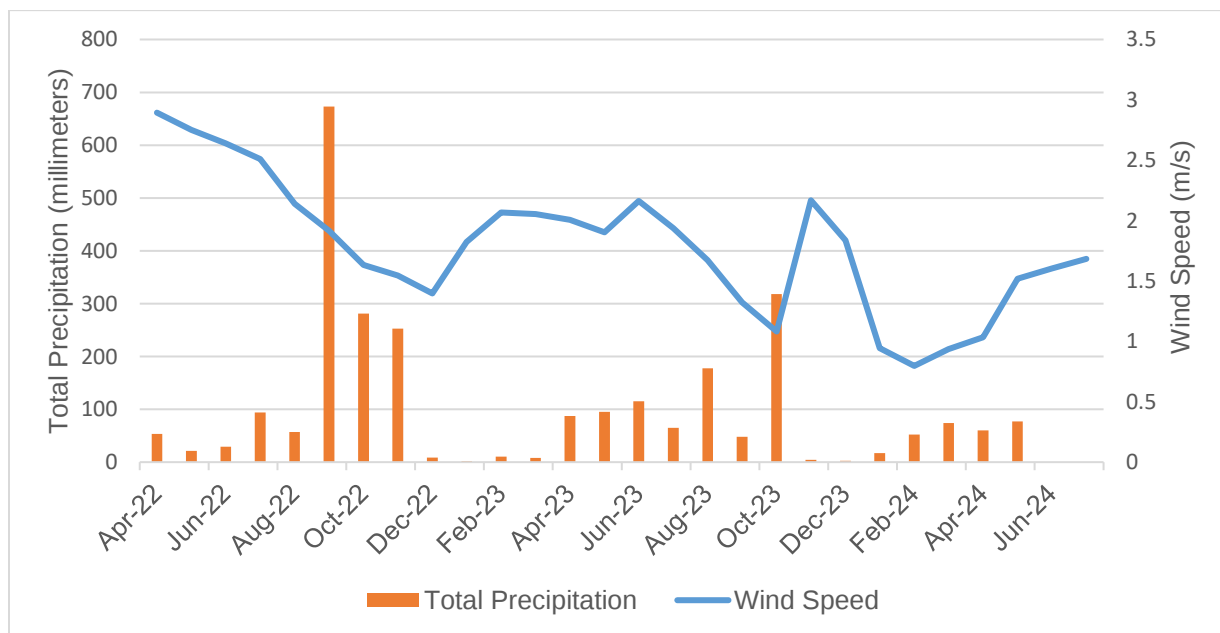
Fig. 2 Graph of monthly total precipitation (millimeters) and average wind speed (m/s) during the study period (April 2022-July 2023).
