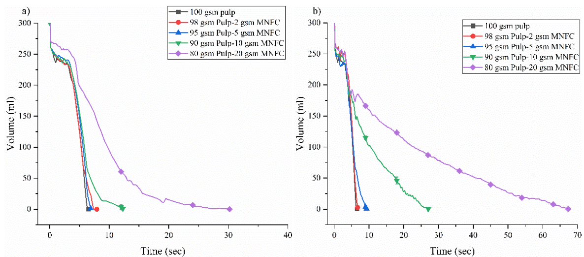
Fig. 1 Volume of furnishes during dewatering of 100 gsm sheets, a) Mixed furnishes b) Multilayer furnish
